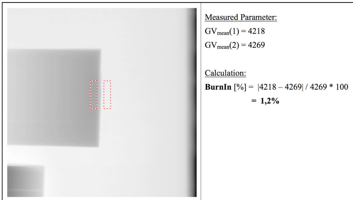
FIG. 9 Measurement of Burn In with the Edge of the Five-Groove Wedge
