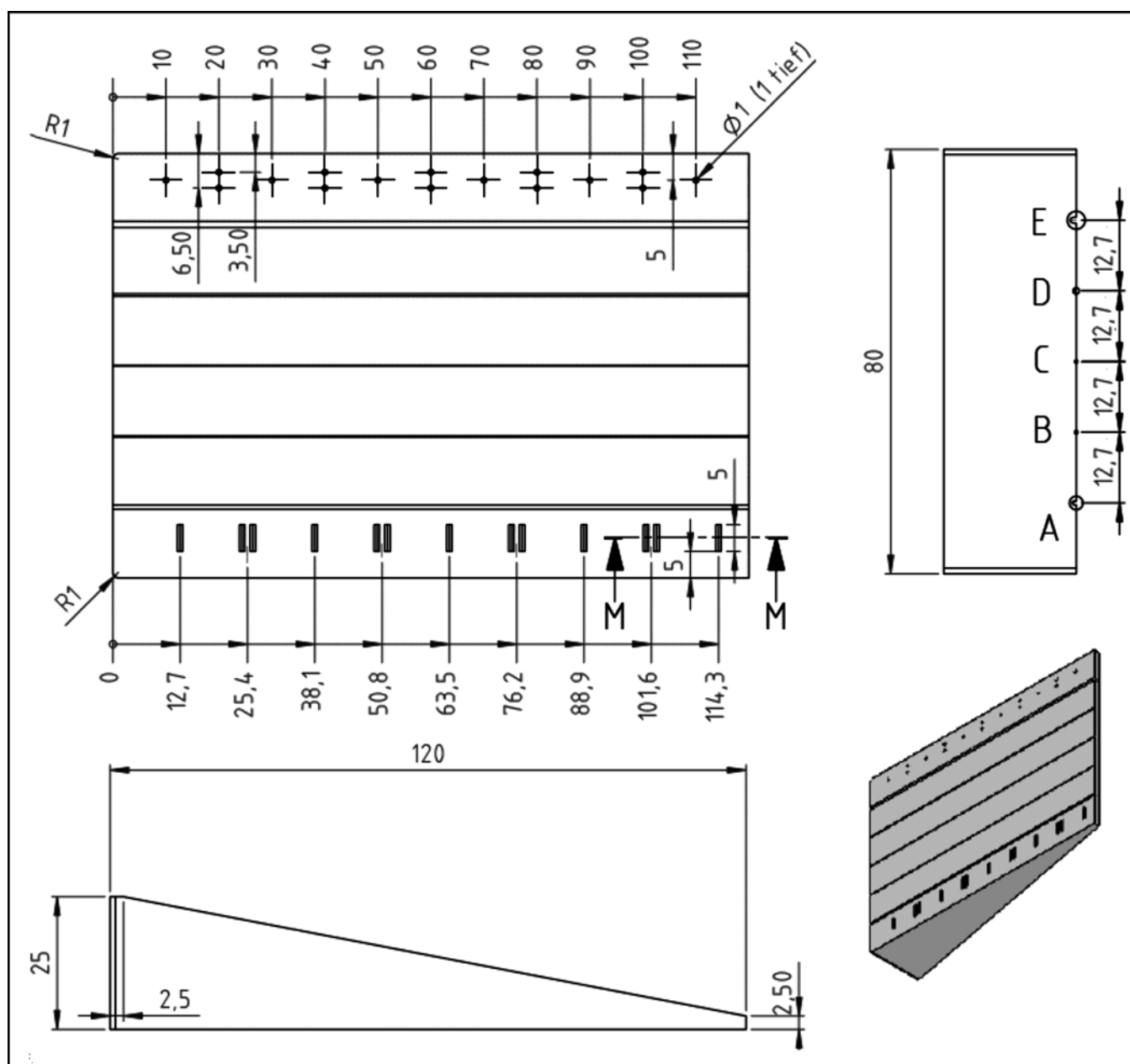
FIG. 1 5-Groove-Wedge (steel) – see Appendix
