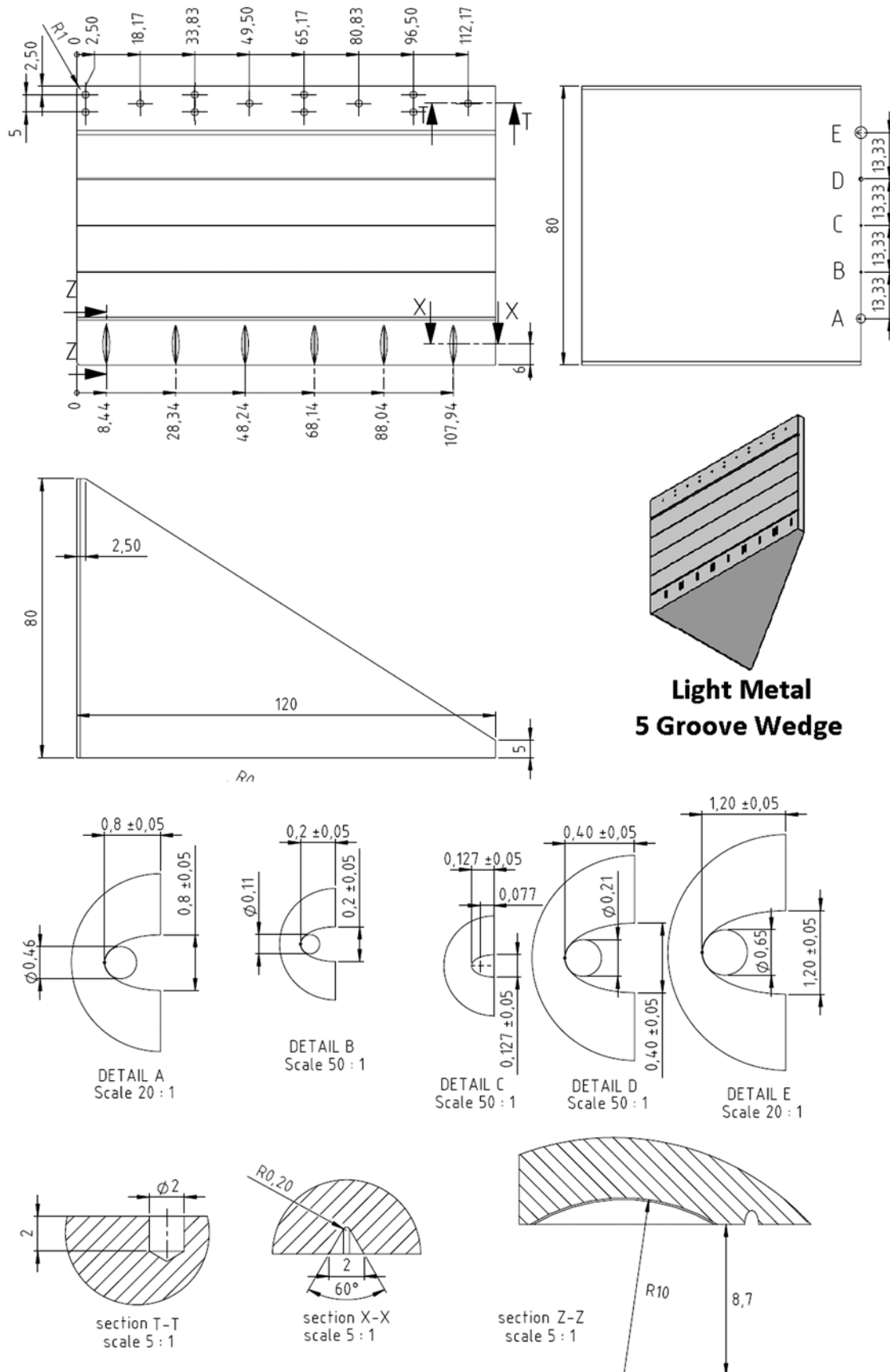
FIG. X1.2 Drawing of F-Groove Wedge for Light Metals
