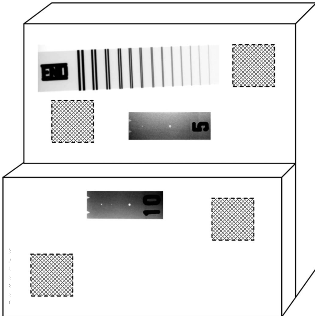
FIG. 2 Duplex Plate Phantom with IQIs positioned; one ASTM E1025 or E1742 Penetrameter on each plate and one ASTM E2002 Duplex Wire IQI on the thinner plate. The boxes ROI 1 to ROI 4 are for evaluation of signal level and SNR.
