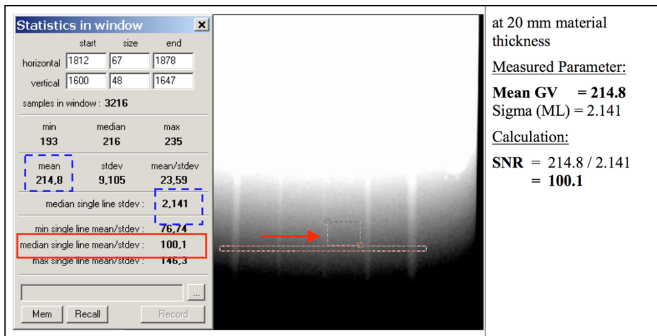
FIG. 4 Measure the Mean Grey Value (Signal Level) and Median Single Line Standard Deviation (Sigma)
