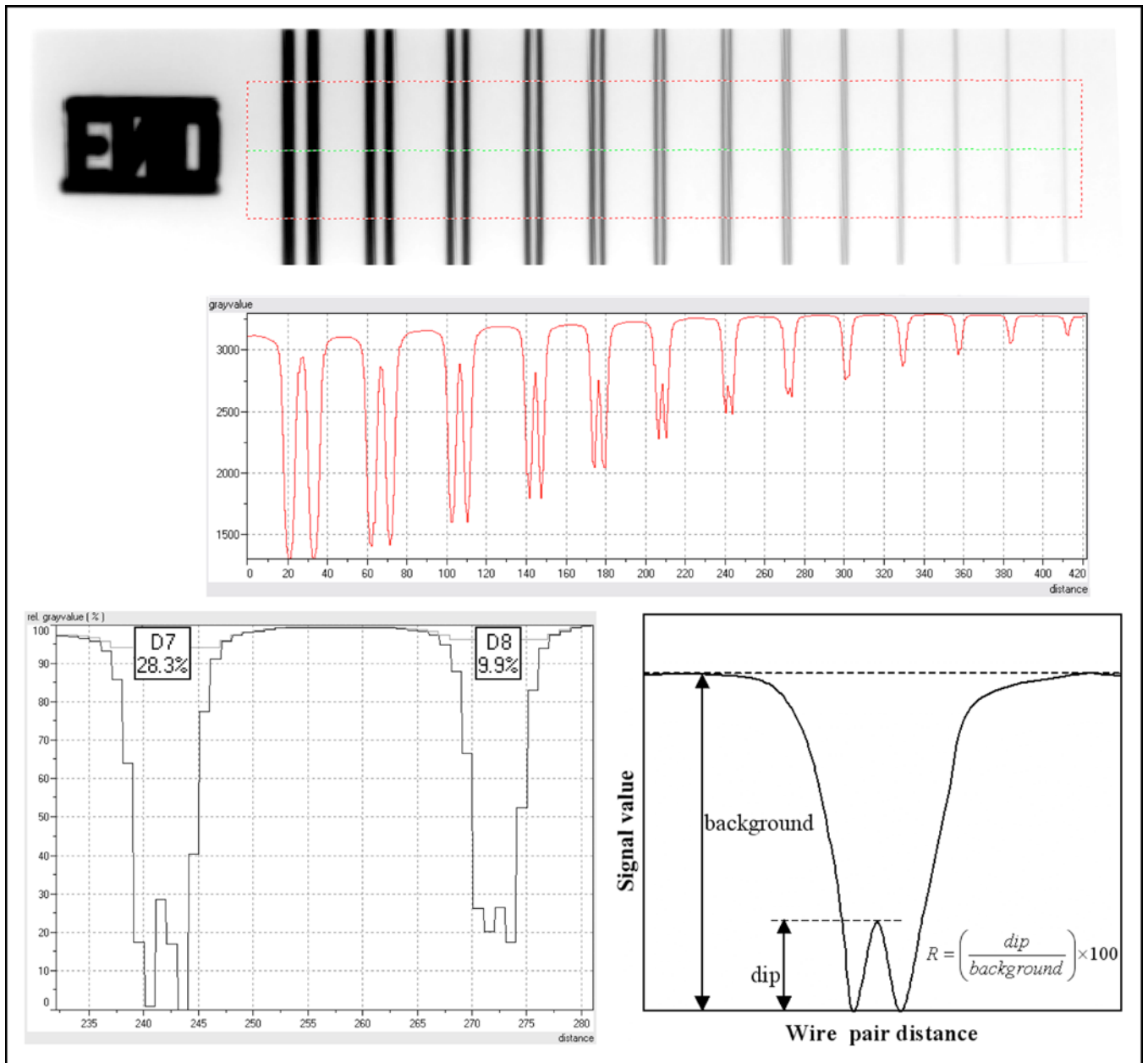
FIG. 6 Wire-Pair Image Analysis for Calculation of Spatial Resolution. D8 < 20 %: 160 \mu m Resolution.
