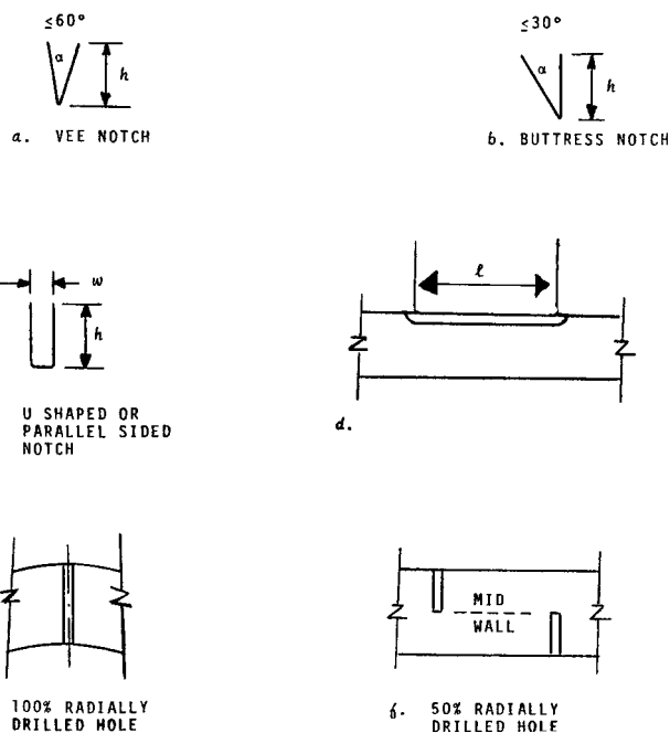
FIG. 3 Common Reference Reflectors
