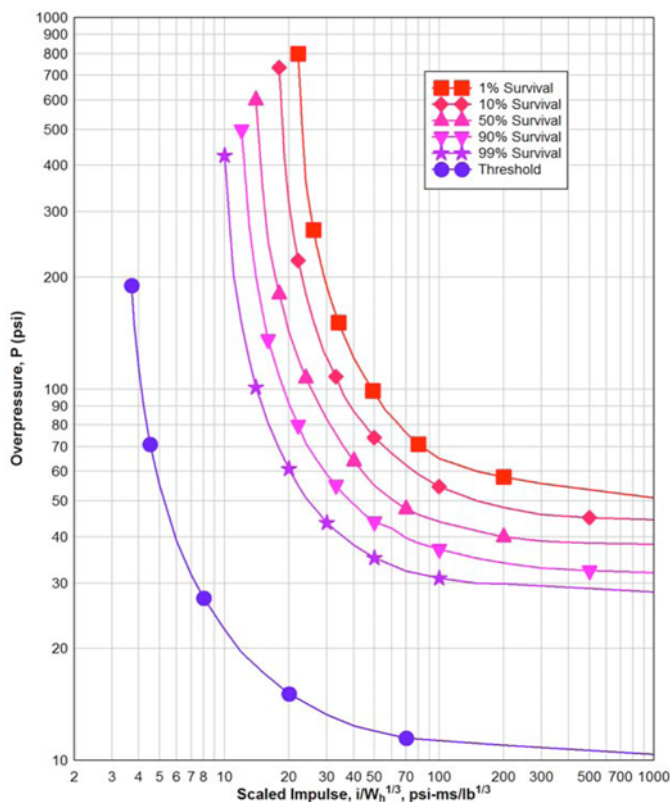
FIG. X1.1 Survivability Curves for Lung Damage From UFC 3-340-02
