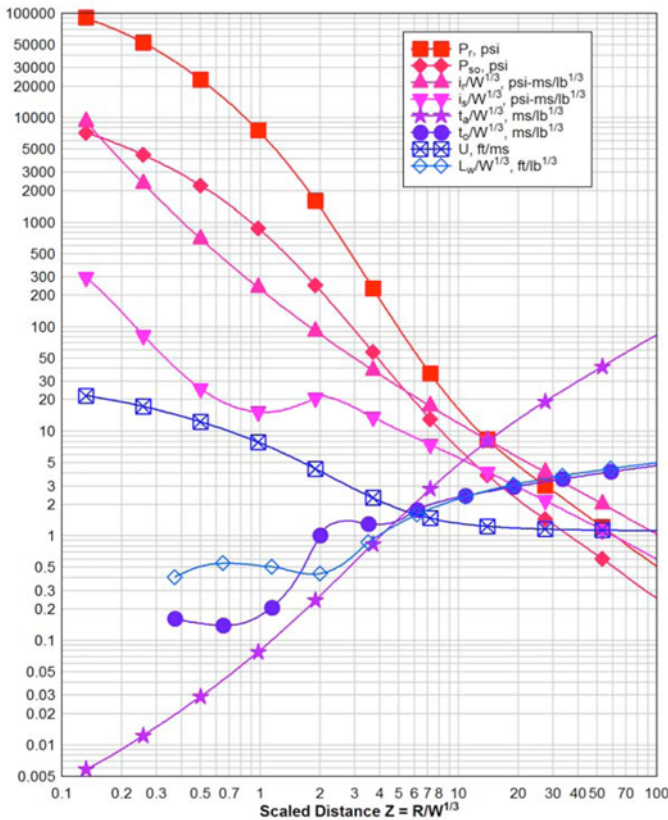
FIG. X1.2 Blast Data Versus Scaled Distance From TM 5-1300
