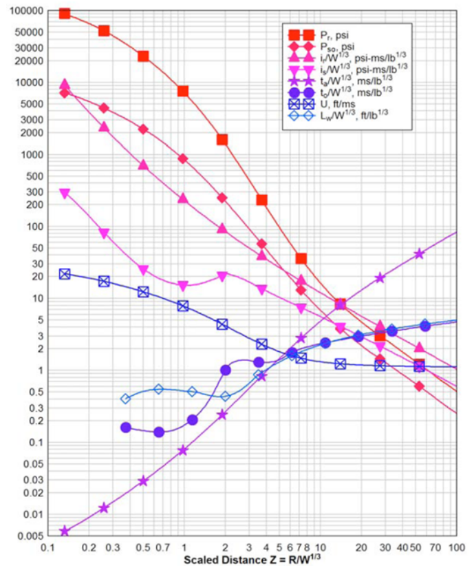
FIG. X1.2 Blast Data Versus Scaled Distance From TM 5-1300
