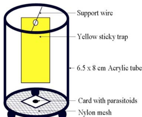
FIG. 1 Test Chamber
