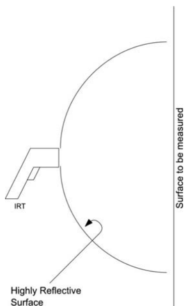
FIG. 8 Gold Cup Measurement
