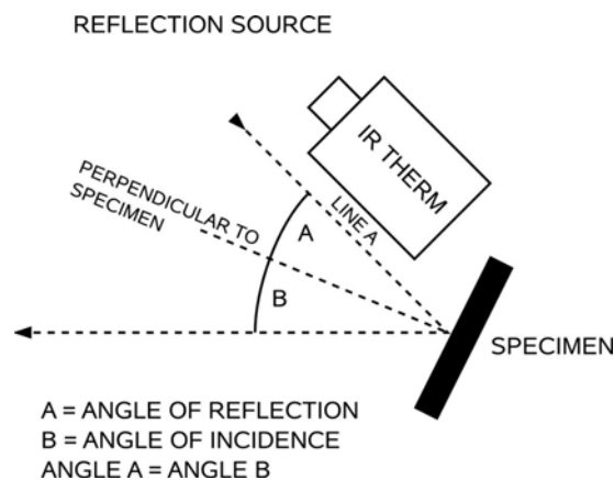
FIG. 11 Testing for Reflected Radiation—Direct Method
