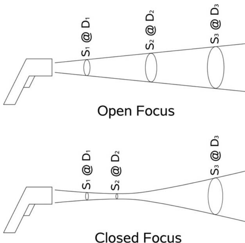
FIG. 6 Distance-to-Size Diagrams
