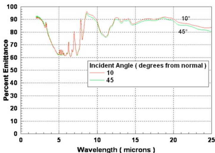
FIG. 4 Example of FTIR Test Results
