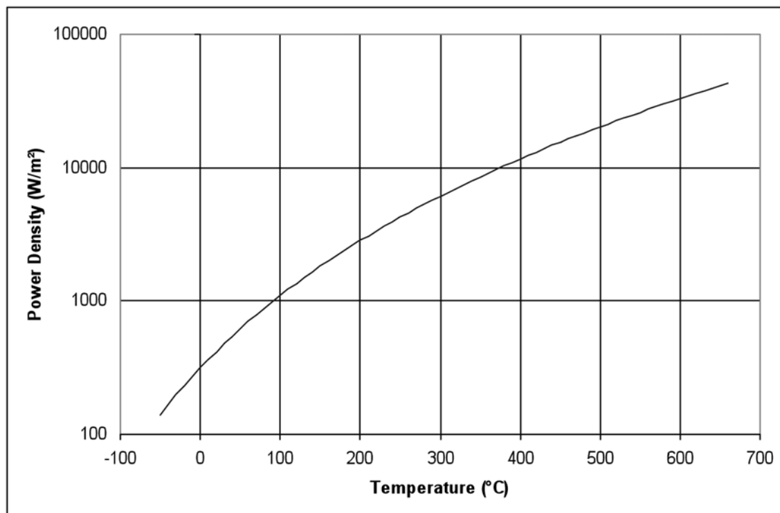
FIG. X1.1 Stefan-Boltzmann Equation
