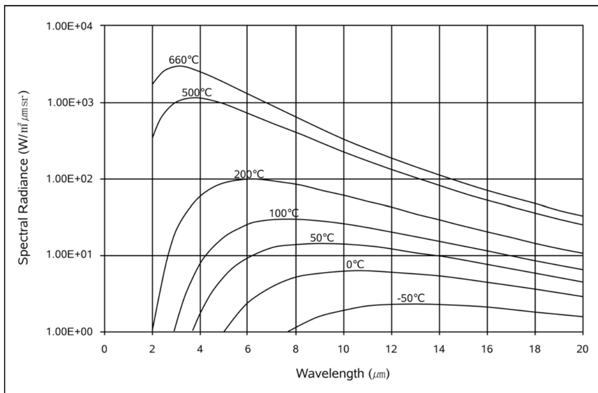
FIG. X1.2 Planck's Law
