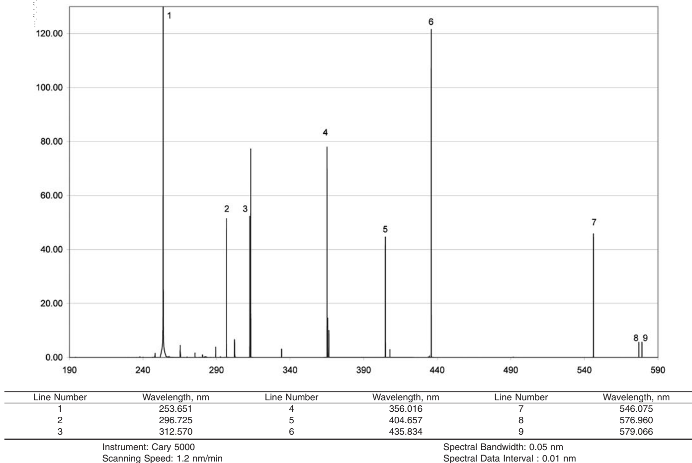
FIG. 1 Mercury Arc Emission Spectrum in the Ultraviolet and Visible Regions Showing Reference Wavelength (4)
