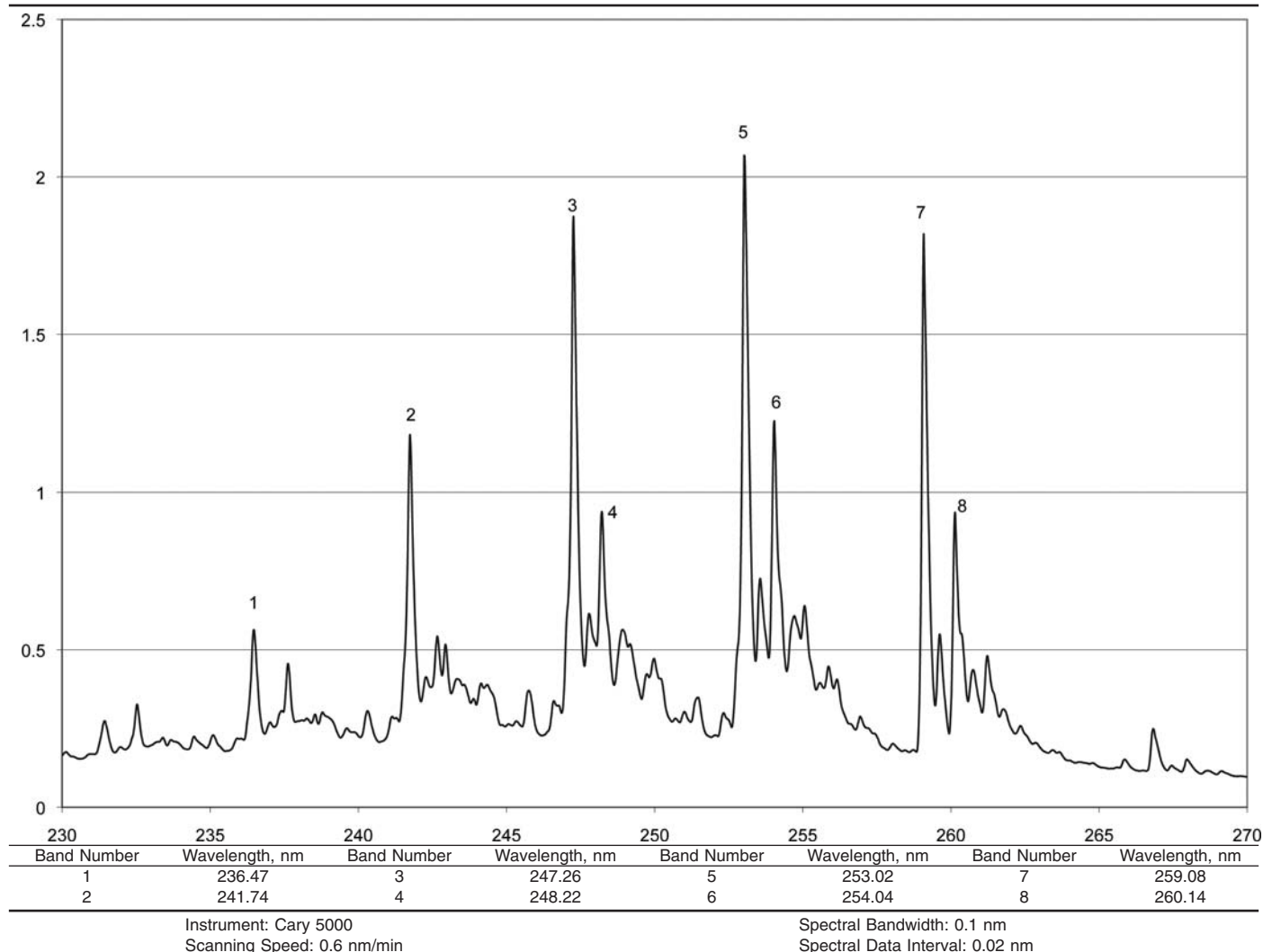
FIG. 4 Spectrum of Benzene Vapor Showing Selected Reference Wavelengths in the Ultraviolet Region (6)
