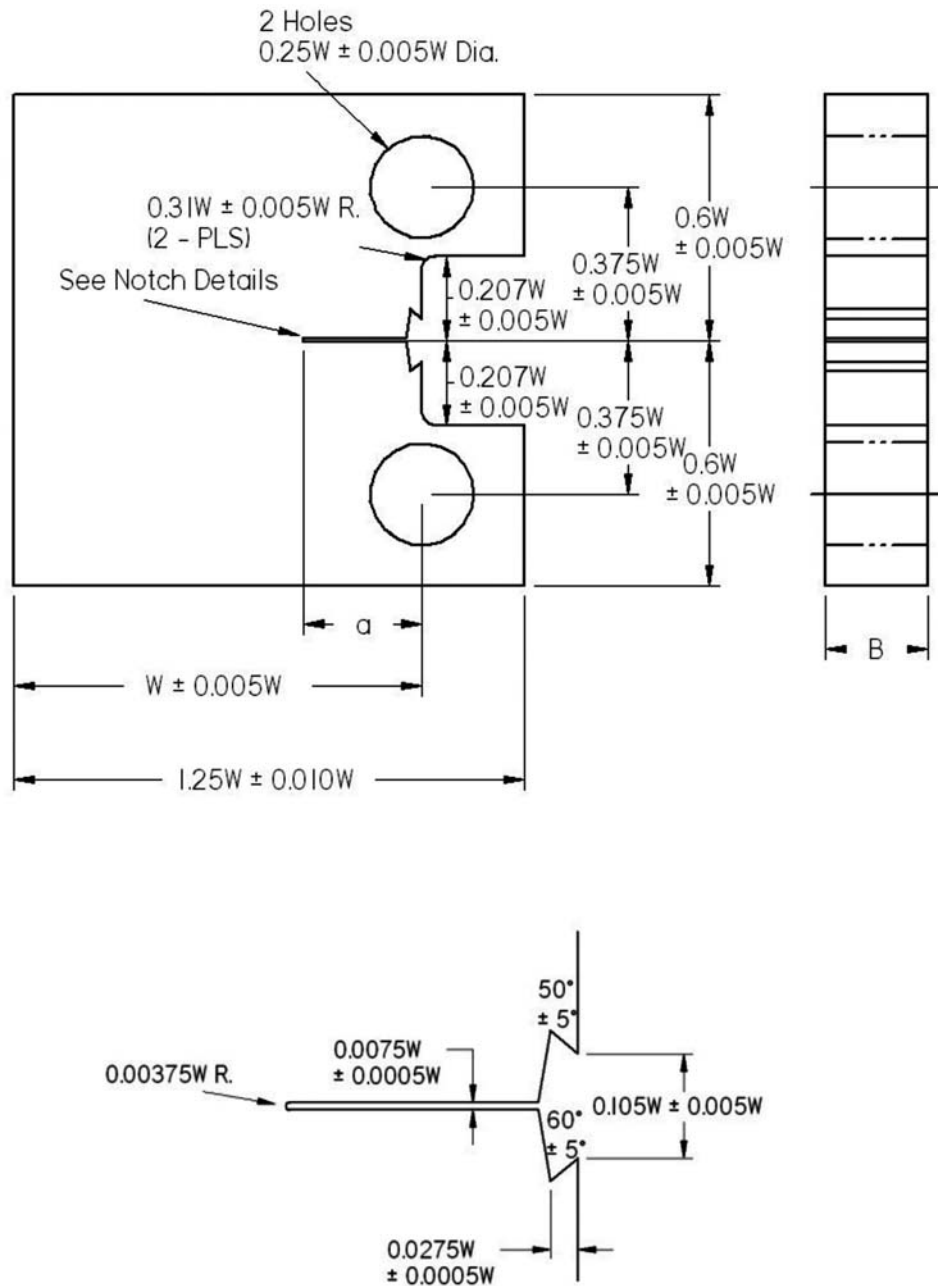
FIG. 1 Drawing of a C(T) Specimen Recommended for Creep-Fatigue Crack Growth Testing and the Details of the Machined Notch and the Knife-Edges for Securely Attaching the Extensometer
