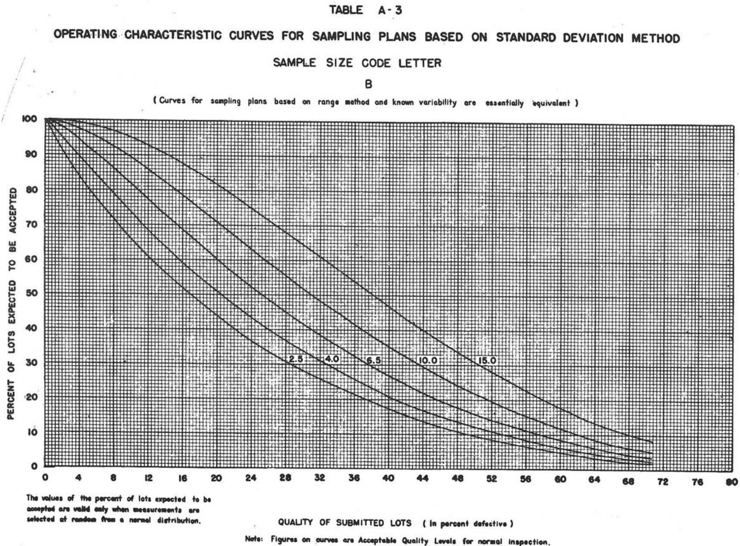
FIG. A1.3 Table A-3 Operating Characteristic Curves for Sampling Plans of Sections 7, 8, and 9
