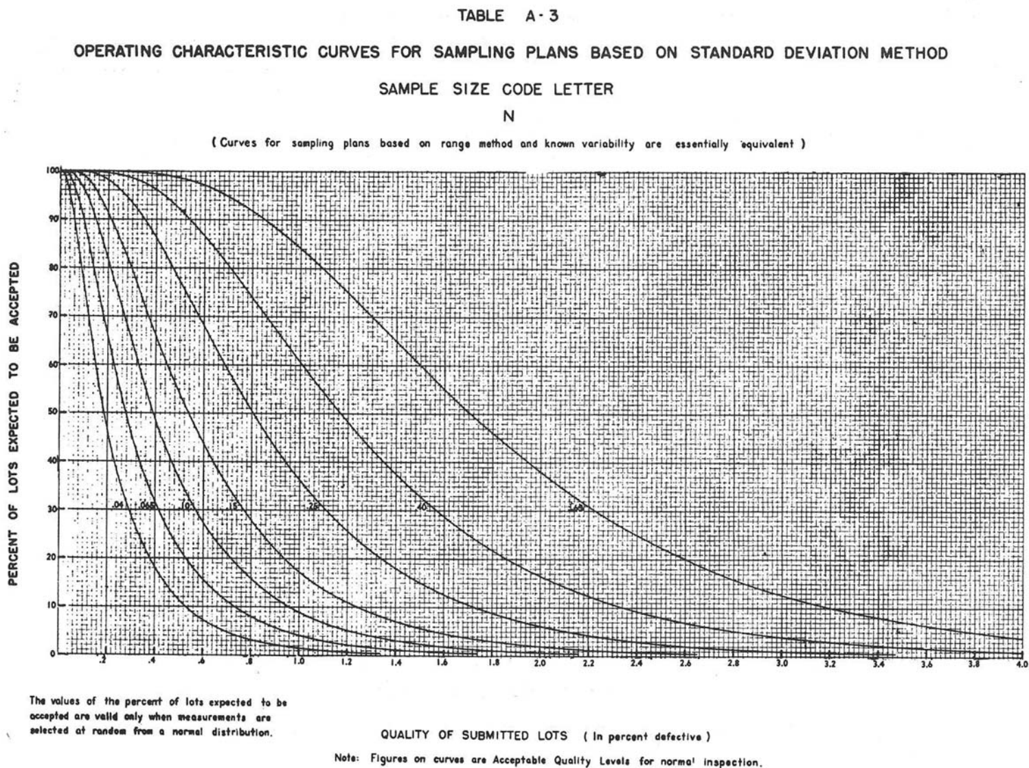
FIG. A1.3 Table A-3 Operating Characteristic Curves for Sampling Plans of Sections 7, 8, and 9 (continued)
