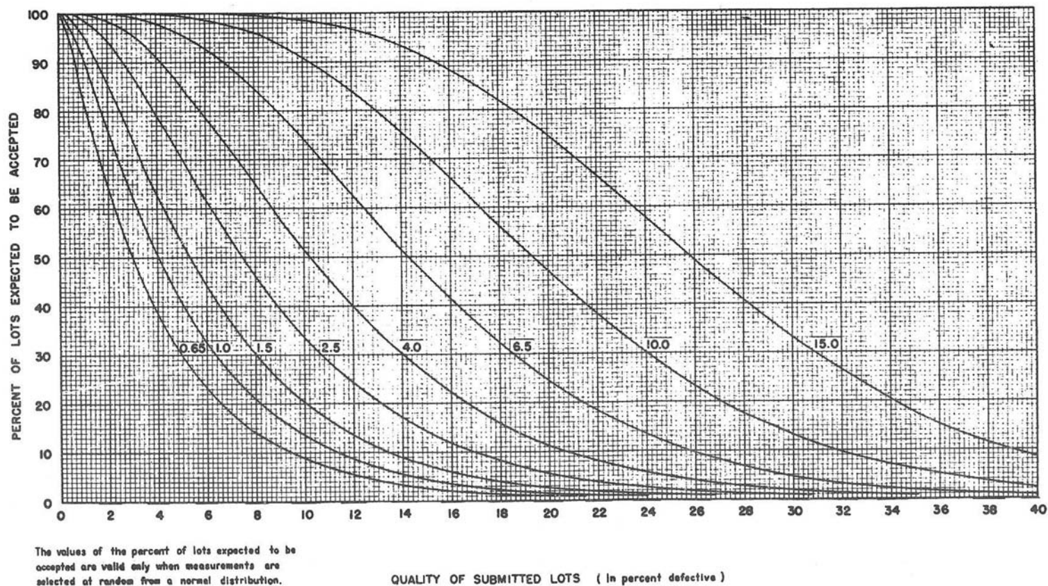
FIG. A1.3 Table A-3 Operating Characteristic Curves for Sampling Plans of Sections 7, 8, and 9 (continued)
