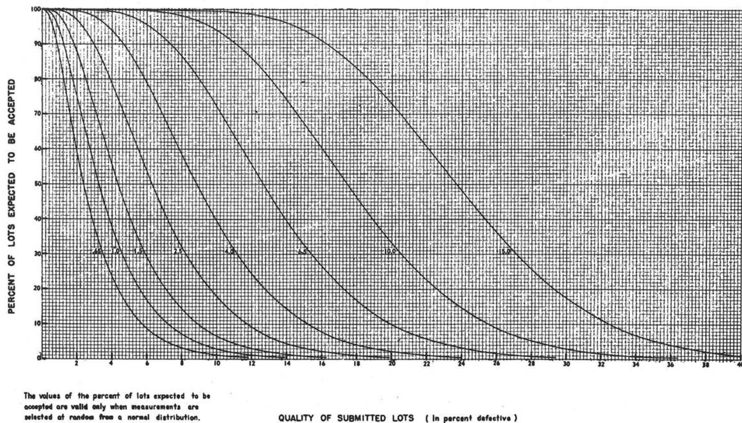
FIG. A1.3 Table A-3 Operating Characteristic Curves for Sampling Plans of Sections 7, 8, and 9 (continued)
