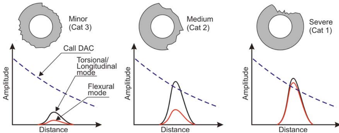
FIG. 3 Illustrations of the Signals in Each Severity Classification
