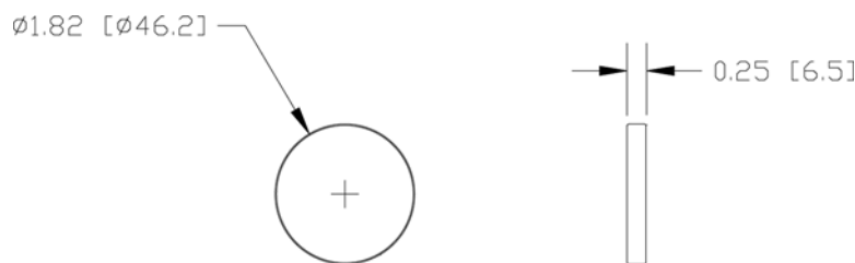
FIG. 2 Restrictor Plate
