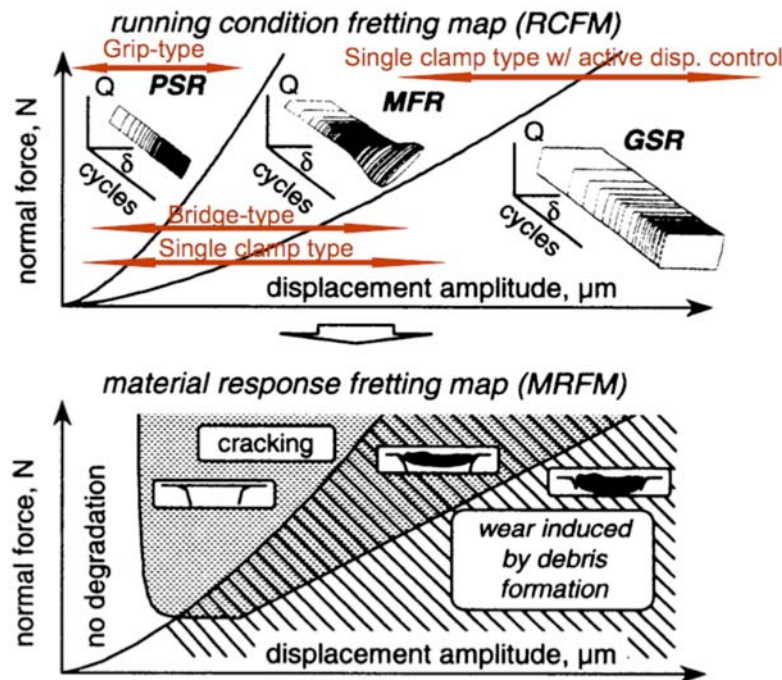
FIG. 2 Fretting Maps
