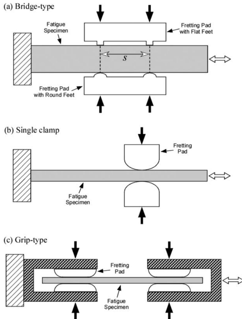
FIG. 5 Fretting Fatigue Test Configurations
