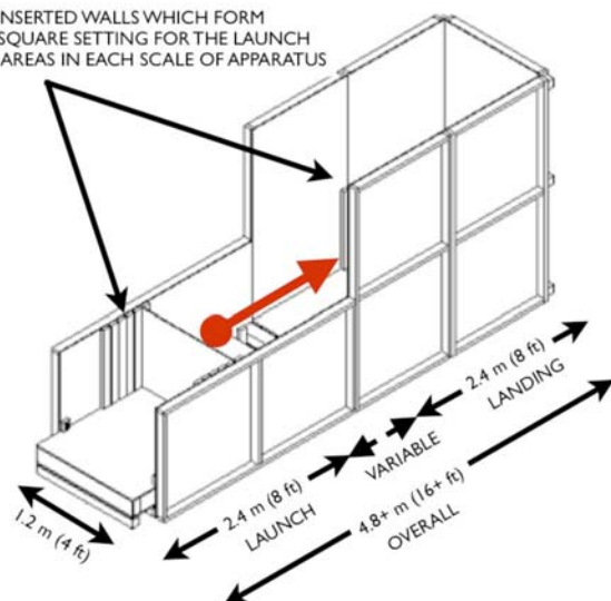
FIG. 2 Mobility: Confined Area Obstacles: Gaps Apparatus (Perspective Views)
