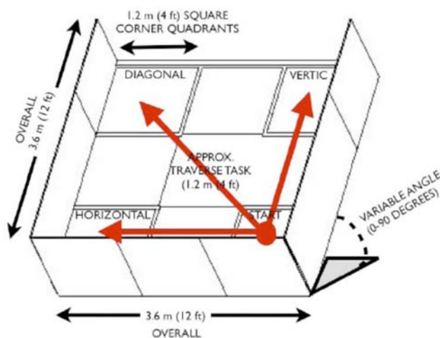
FIG. 2 Mobility: Confined Area Obstacles: Inclined Planes Apparatus (Perspective Views)
