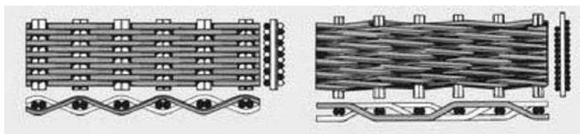
FIG. 1 Double Warp Plain and Double Warp Twill Weave
