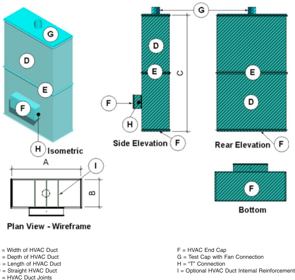
FIG. 2 Condition B – Vertical HVAC Duct without Openings
