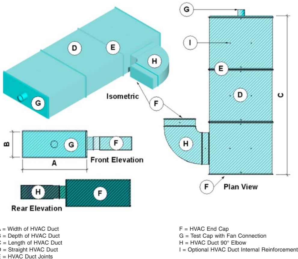
FIG. 1 Condition A – Horizontal HVAC without Openings
