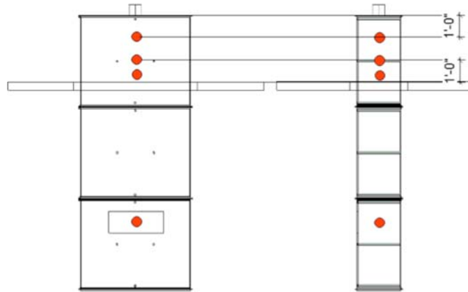
FIG. 17 Unexposed Thermocouple Inside Duct – Front and Side View of Vertical Test Assembly
