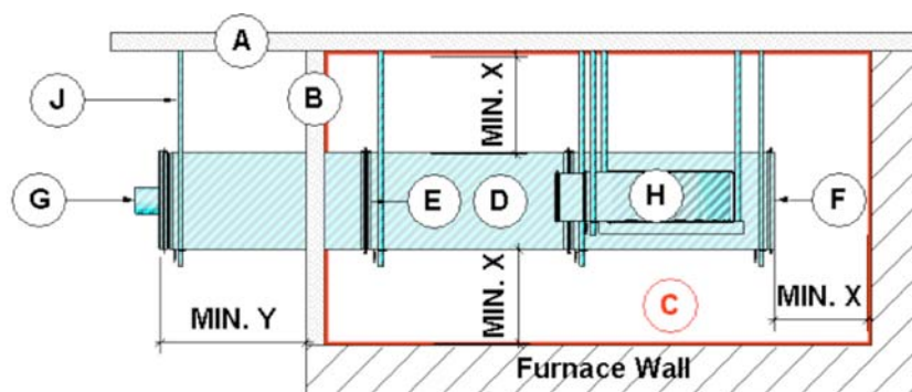
FIG. 6 Plan View of Test Assembly Condition A – Horizontal HVAC Duct without Openings
