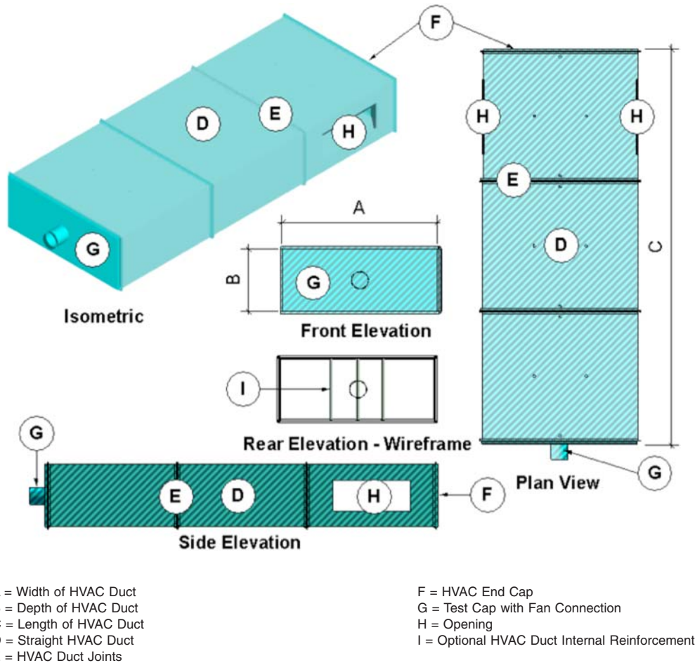
FIG. 3 Condition C – Horizontal HVAC Duct with Openings
