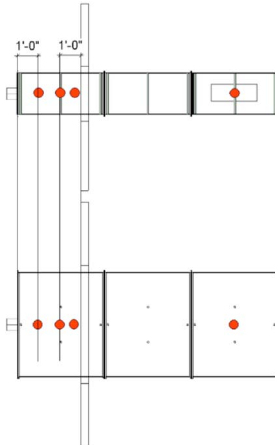
FIG. 18 Unexposed Thermocouple Inside Duct – Top and Side View of Horizontal Test Assembly
