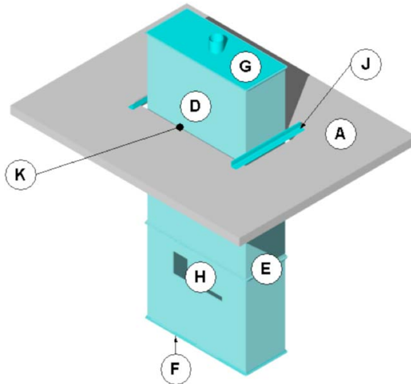
FIG. 13 Side View of Test Assembly Condition C – Horizontal HVAC Duct with Openings
