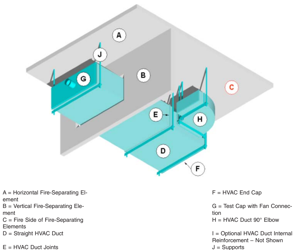
FIG. 5 Isometric View of Test Assembly Condition A – Horizontal HVAC Duct without Openings
