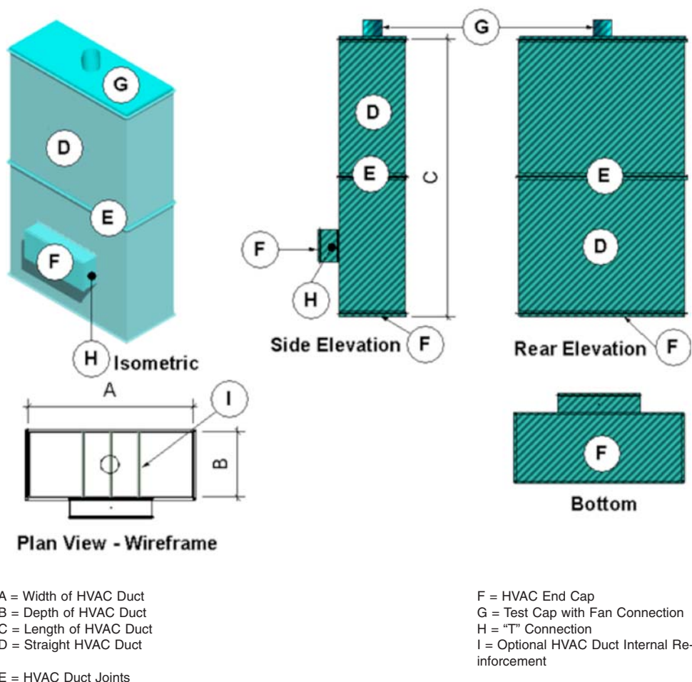
FIG. 2 Condition B – Vertical HVAC Duct without Openings
