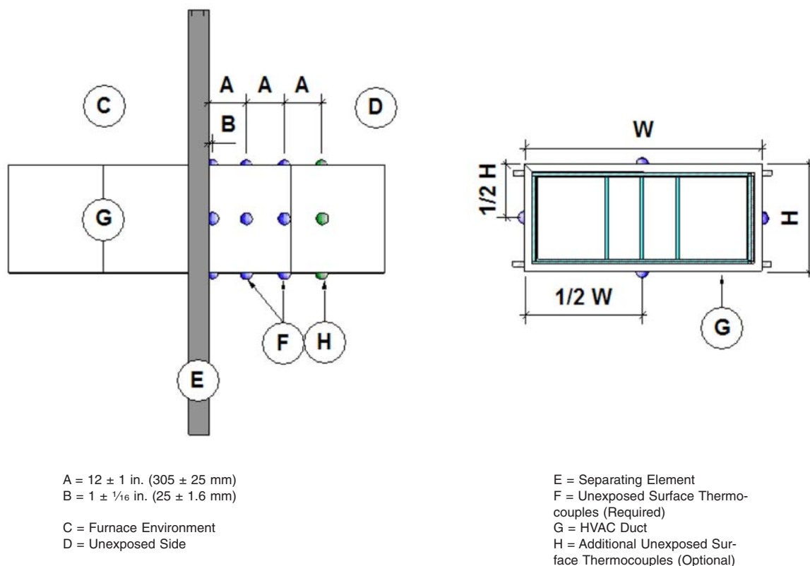
FIG. 19 Unexposed Surface Thermocouples Locations on HVAC Duct – Horizontal and Vertical Test Assemblies
