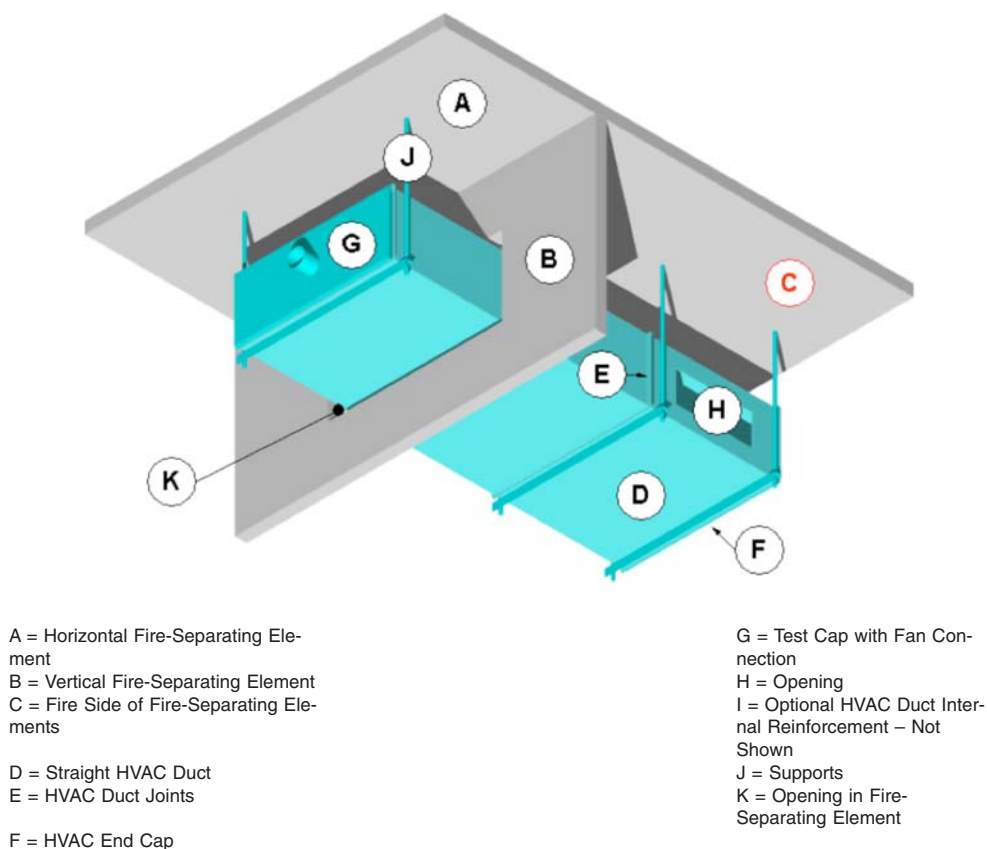
FIG. 11 Isometric View of Test Assembly Condition C – Horizontal HVAC Duct with Openings
