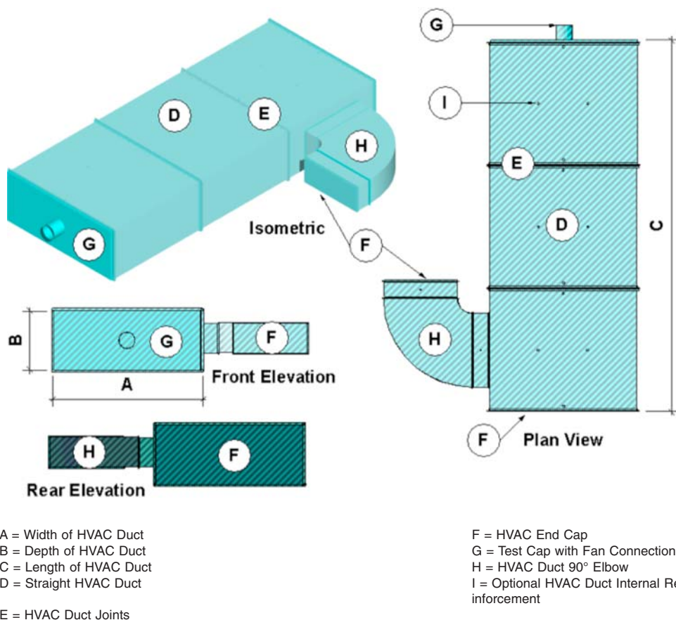
FIG. 1 Condition A – Horizontal HVAC without Openings
