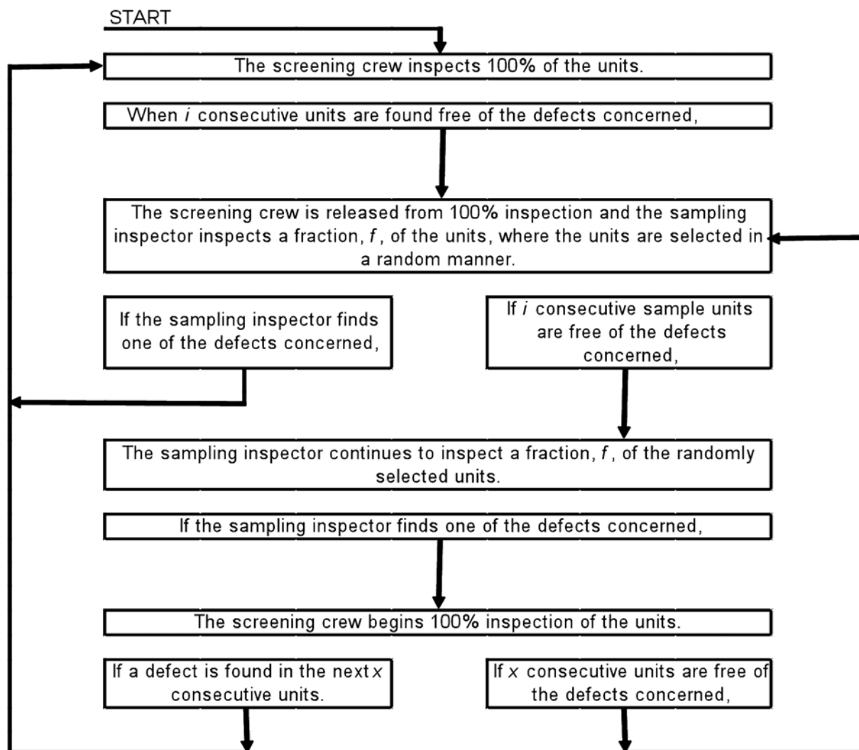
FIG. A1.5 Procedure for CSP-V Plans
