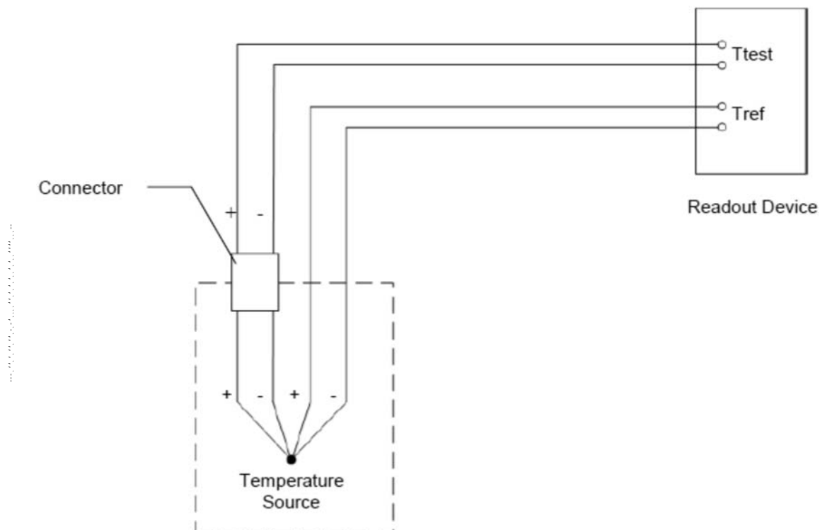
FIG. 1 Test Schematic Using a Readout Device with Cold Junction Compensation, Providing Temperature Indications of the Test Thermocouple T_{\text{test}} and Reference Thermocouple T_{\text{ref}}
