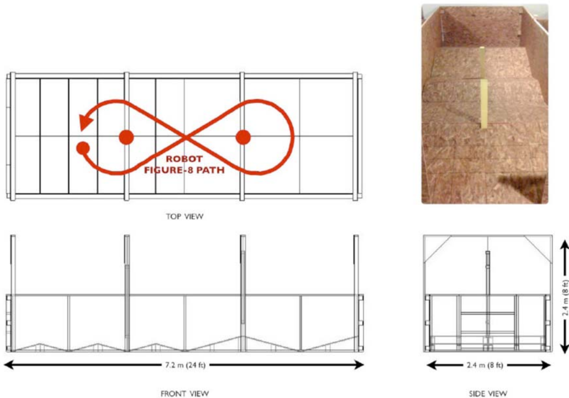
FIG. 4 Mobility: Confined Area Terrains: Continuous Pitch/Roll Ramps Apparatuses (Projection View)
