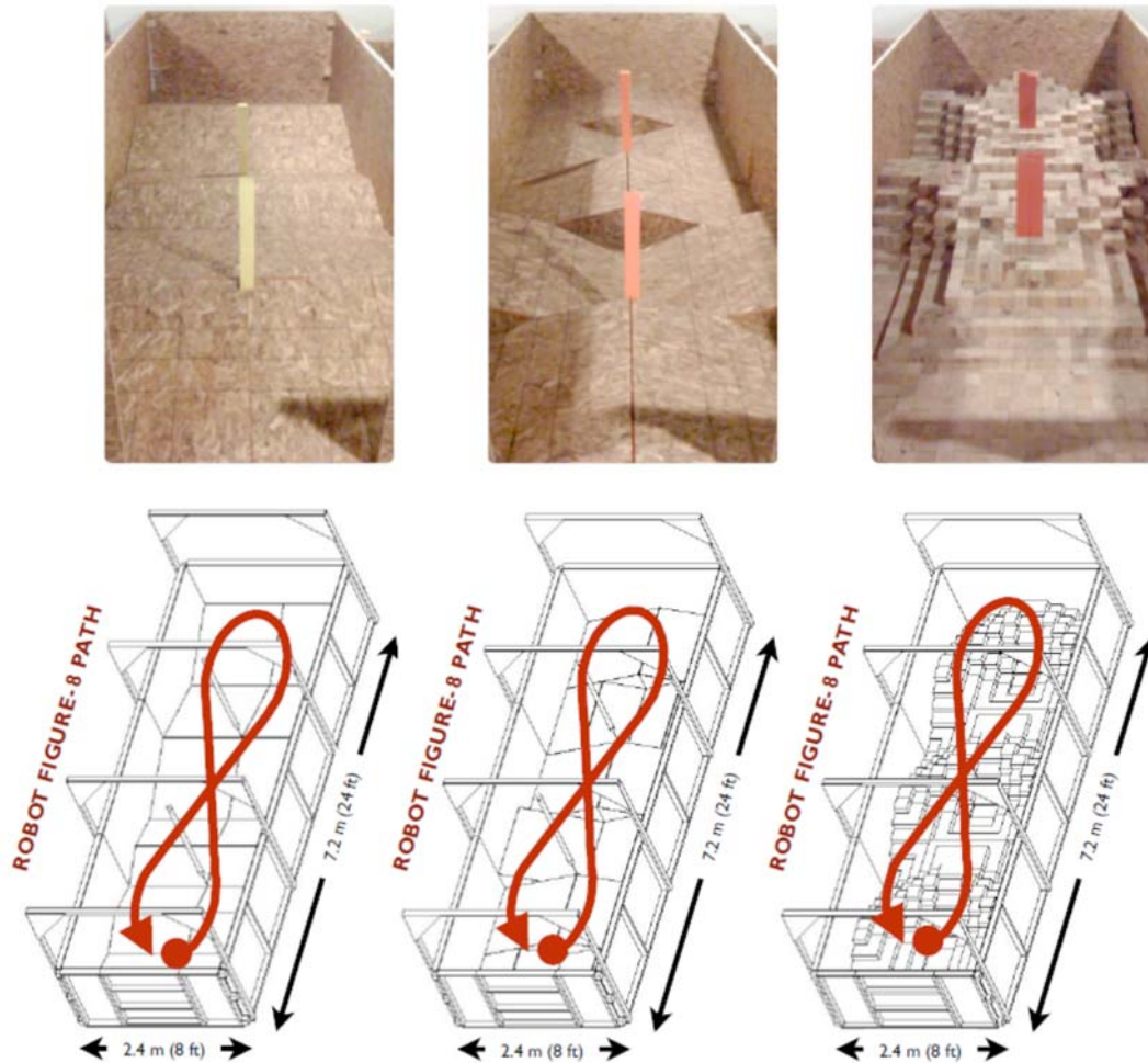
FIG. 2 Three Confined Area Terrain Apparatuses in the Mobility Test Suite with Increasing Complexity; The Continuous Pitch/Roll Ramps Terrain is Shown on the Left. The Crossing Pitch/Roll Ramps is Shown at the Center. The Symmetric Stepfields Terrain is Shown on the Right.
