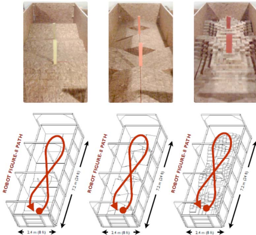
FIG. 2 Three Confined Area Terrain Apparatuses in the Mobility Test Suite with Increasing Complexity; The Continuous Pitch/Roll Ramps Terrain is Shown on the Left. The Crossing Pitch/Roll Ramps Terrain is Shown at the Center. The Symmetric Stepfields Terrain is Shown on the Right.
