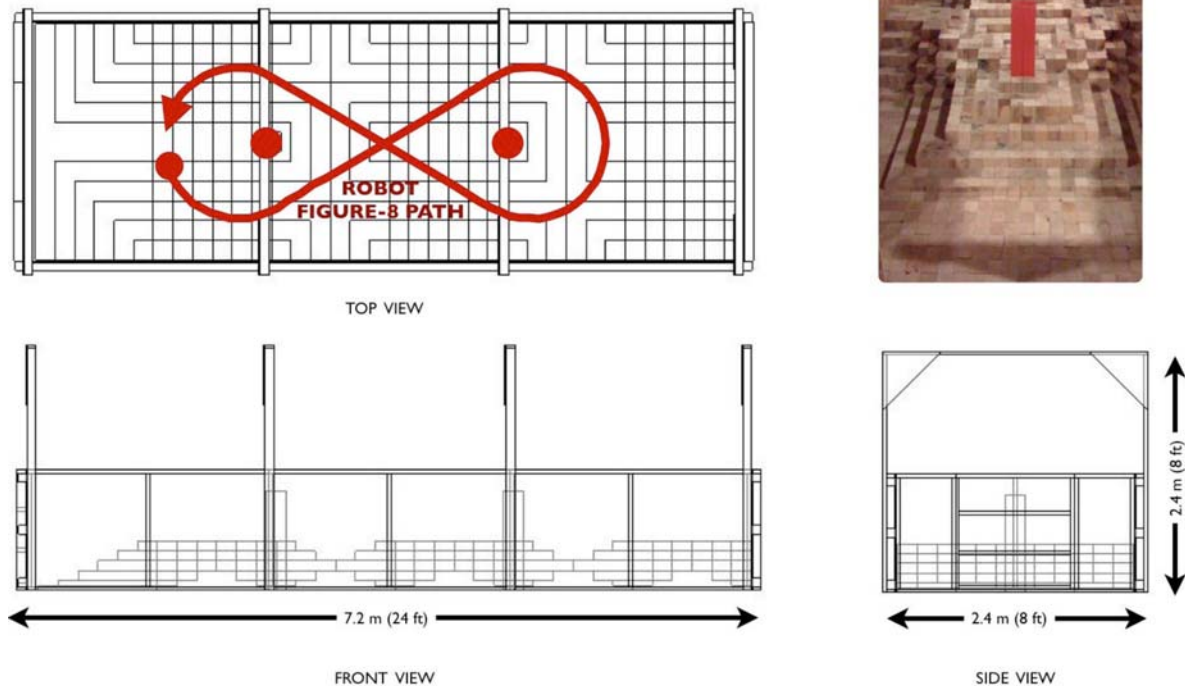
FIG. 4 Mobility: Confined Area Terrains: Symmetric Stepfield Apparatuses (Projection View)
