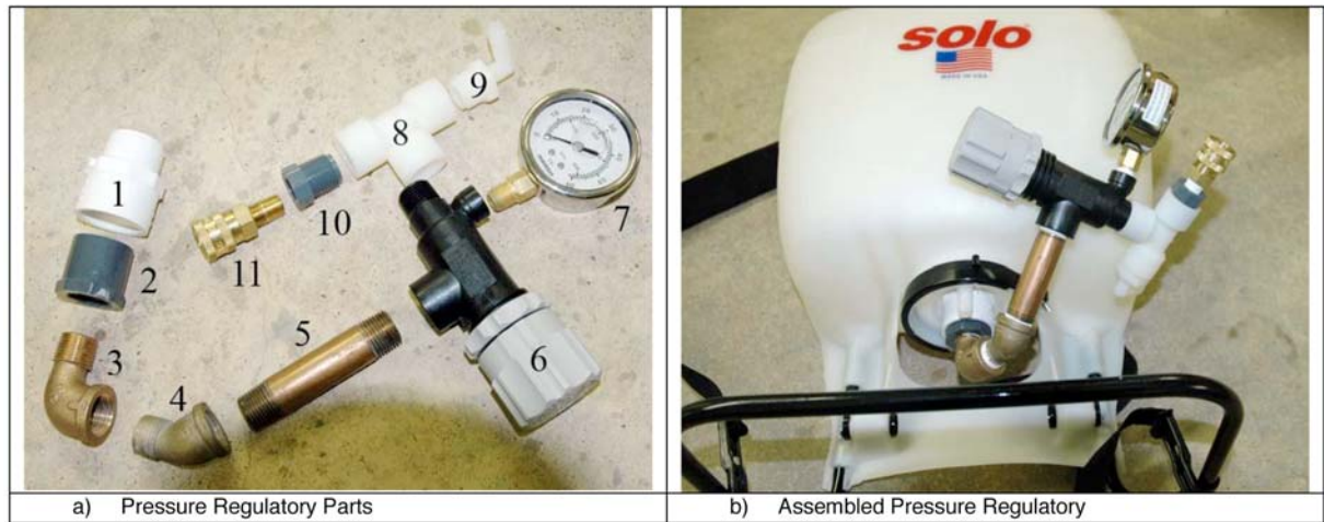
FIG. A1.2 Pressure Regulatory Assembly
