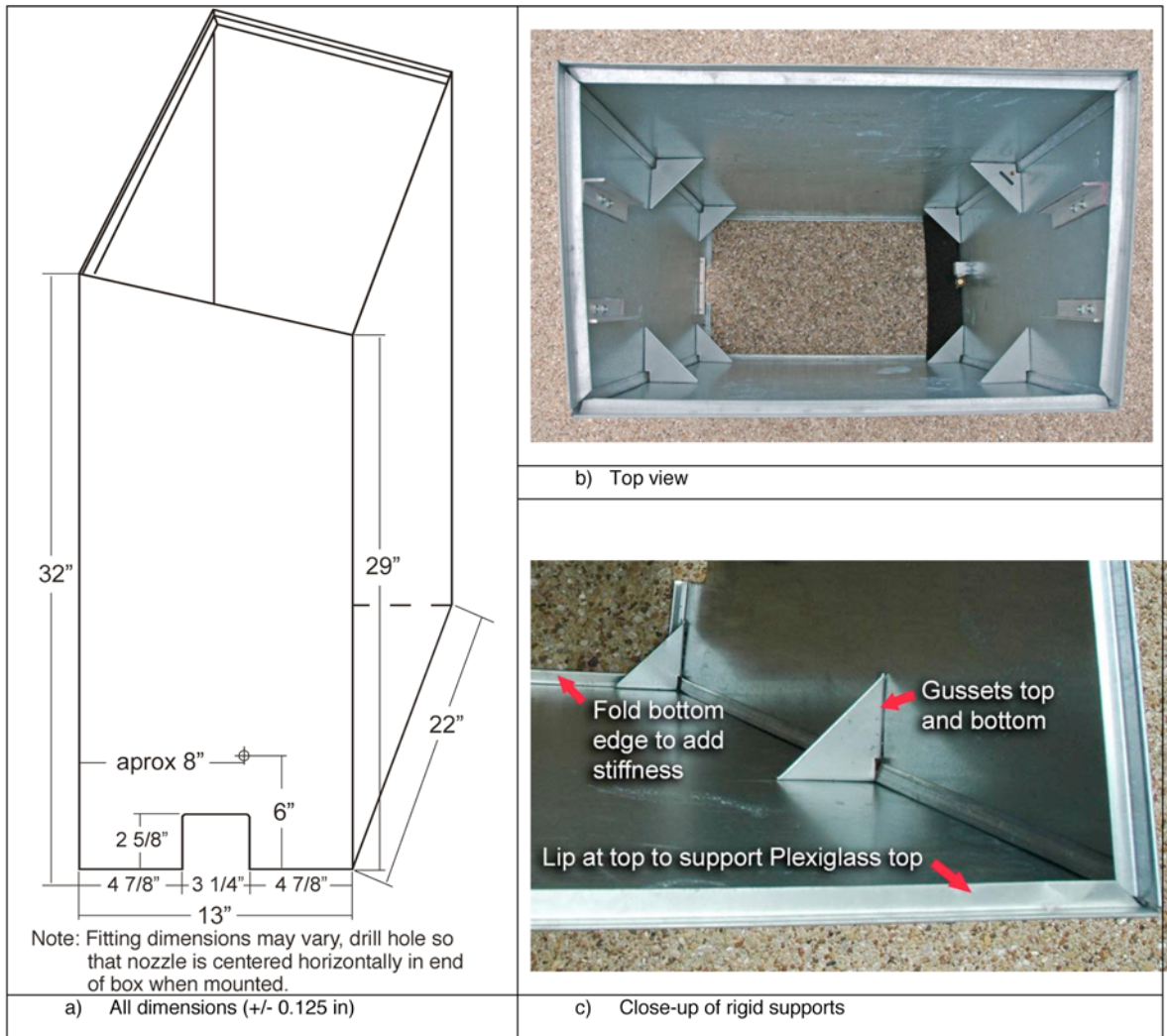
FIG. A1.6 Spray Box Design
