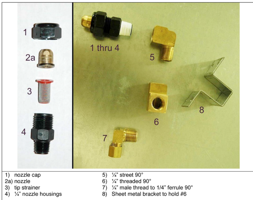
FIG. A1.7 Spray Nozzle Assembly
