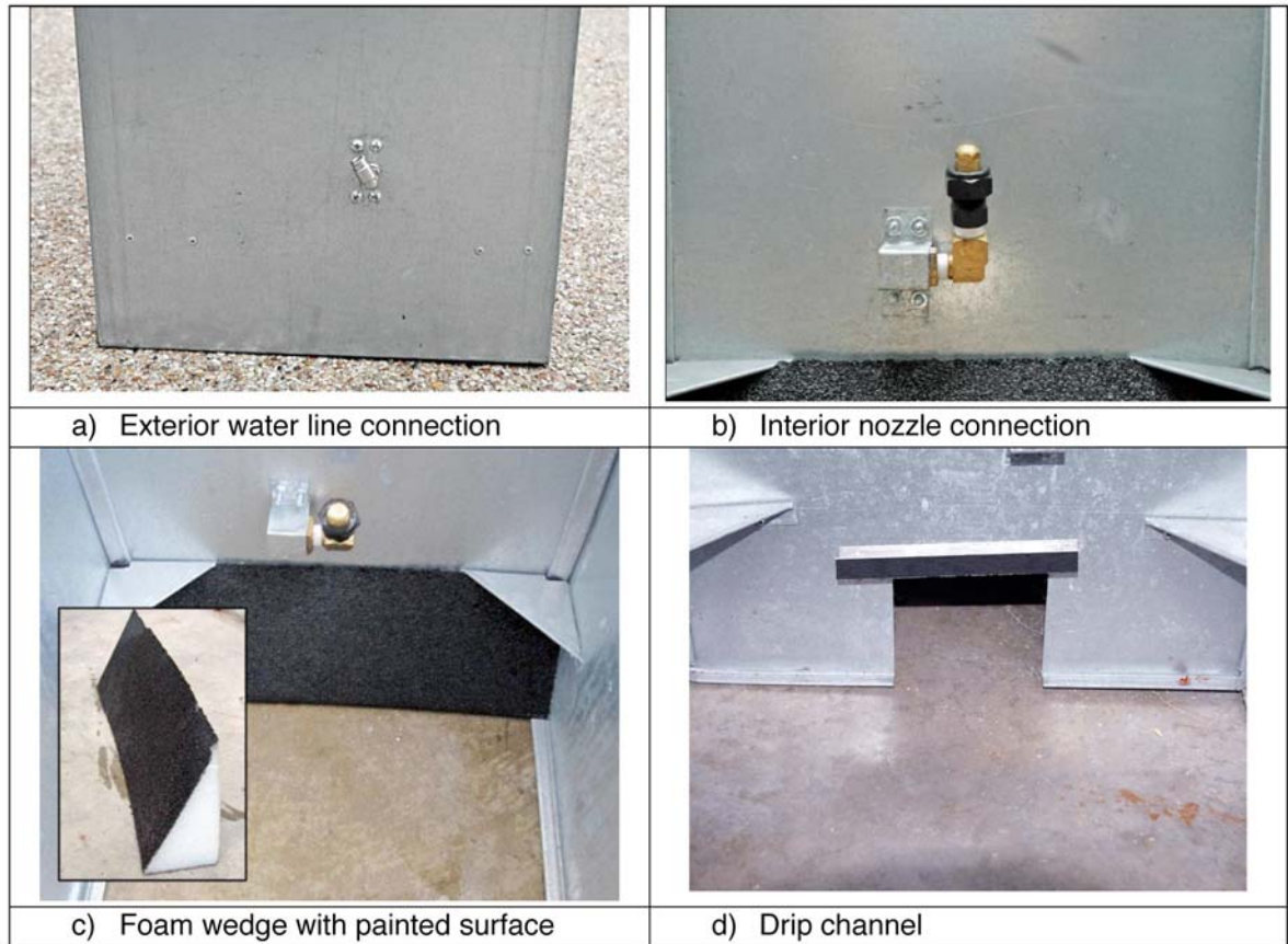
FIG. A1.8 Spray Nozzles Installation
