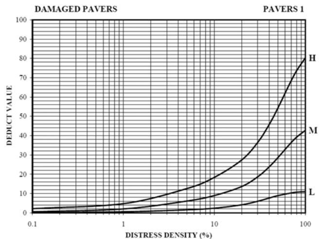
FIG. X3.1 Damaged Pavers (1)
