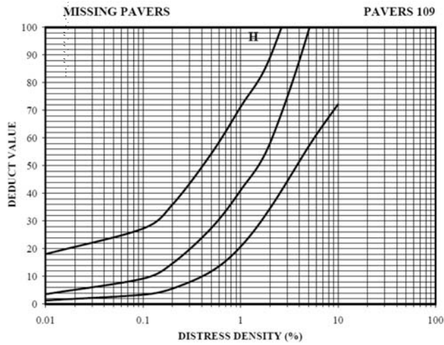
FIG. X3.9 Missing Pavers (9)
