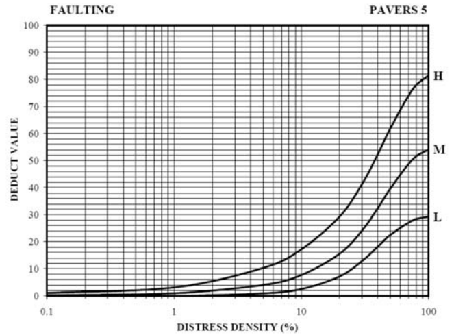
FIG. X3.5 Faulting (5)
