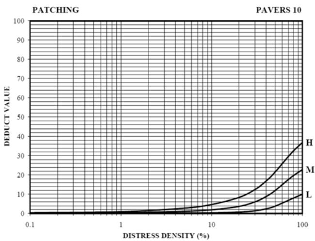
FIG. X3.10 Patching (10)
