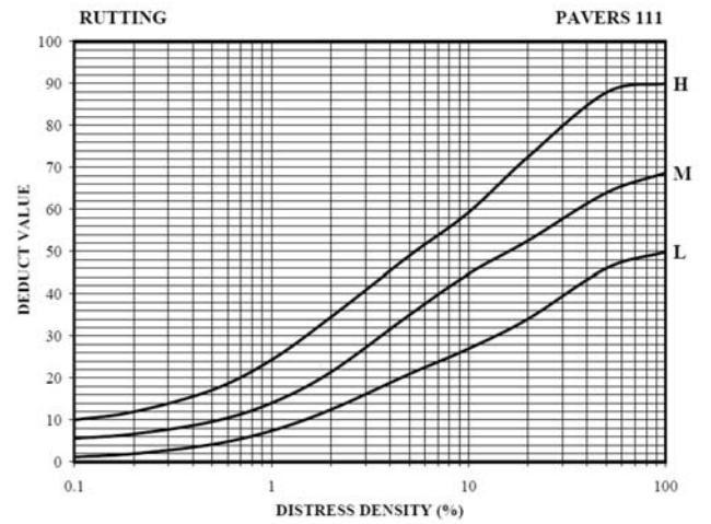
FIG. X3.11 Rutting (11)
