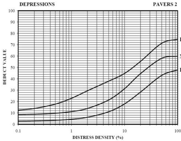
FIG. X3.2 Depressions (2)
