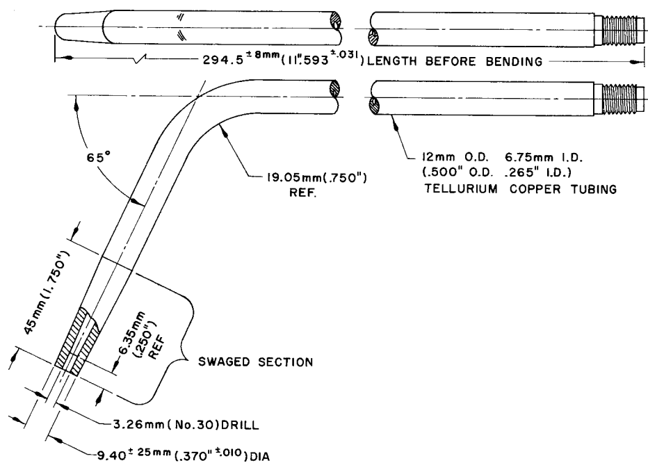
FIG. 4 Victor Type 4, No. 7 Torch Tip
