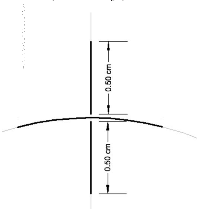
FIG. 4 Cadmium Cross Construction: Insert the 1.0-cm long piece of cadmium wire into the circular groove at each cross location depicted in Fig. 3. Place one of the 0.5-cm long cadmium pieces on either side of it in the radial groove, ensuring that all of the wires remain in the grooves.
