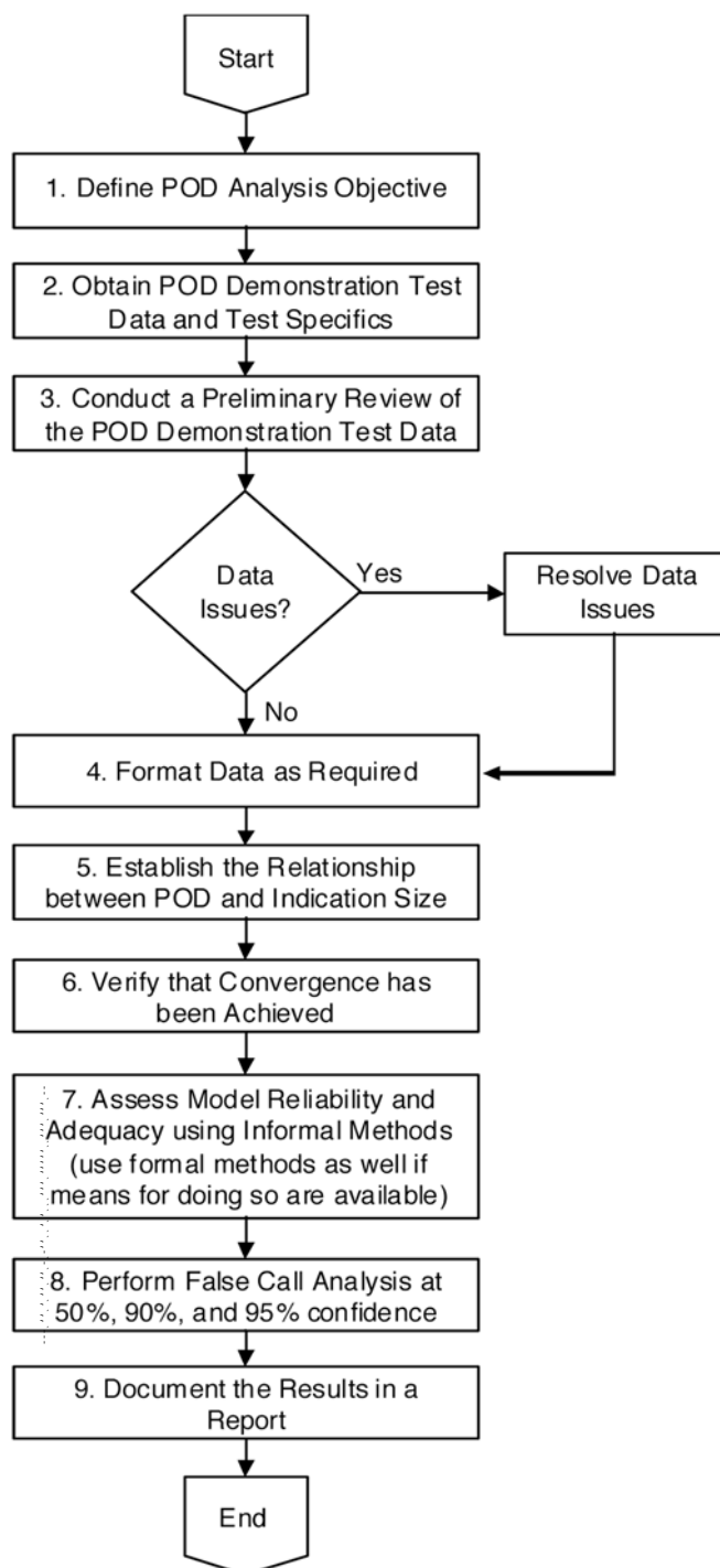
FIG. X1.1 Flowchart of POD Analysis for Hit/Miss Data
