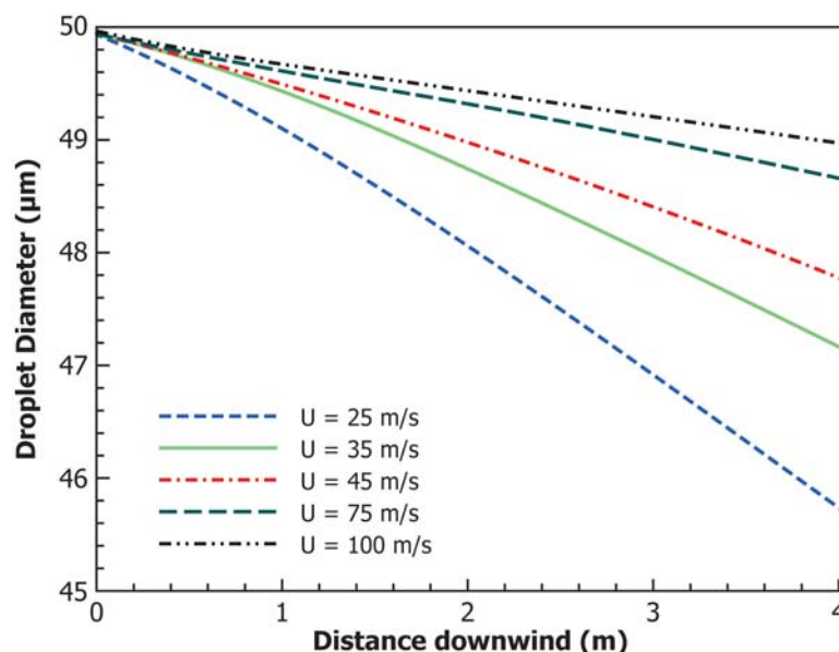
FIG. 3 Diameter Reduction of a 50- \mu\text{m} Droplet Released from Rest in a Uniform Airstream at 20°C and 50 % Relative Humidity
