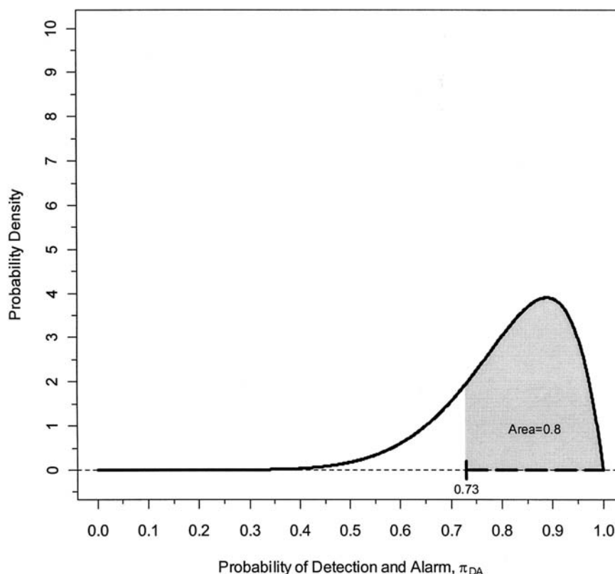
FIG. X2.4 Statistical Results after Observing Nine Tests in which Only Eight Tests Resulted in Detection and Alarm
