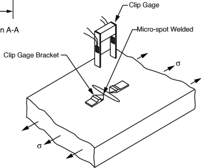
FIG. X3.1 Attachment methods for CMOD gages
