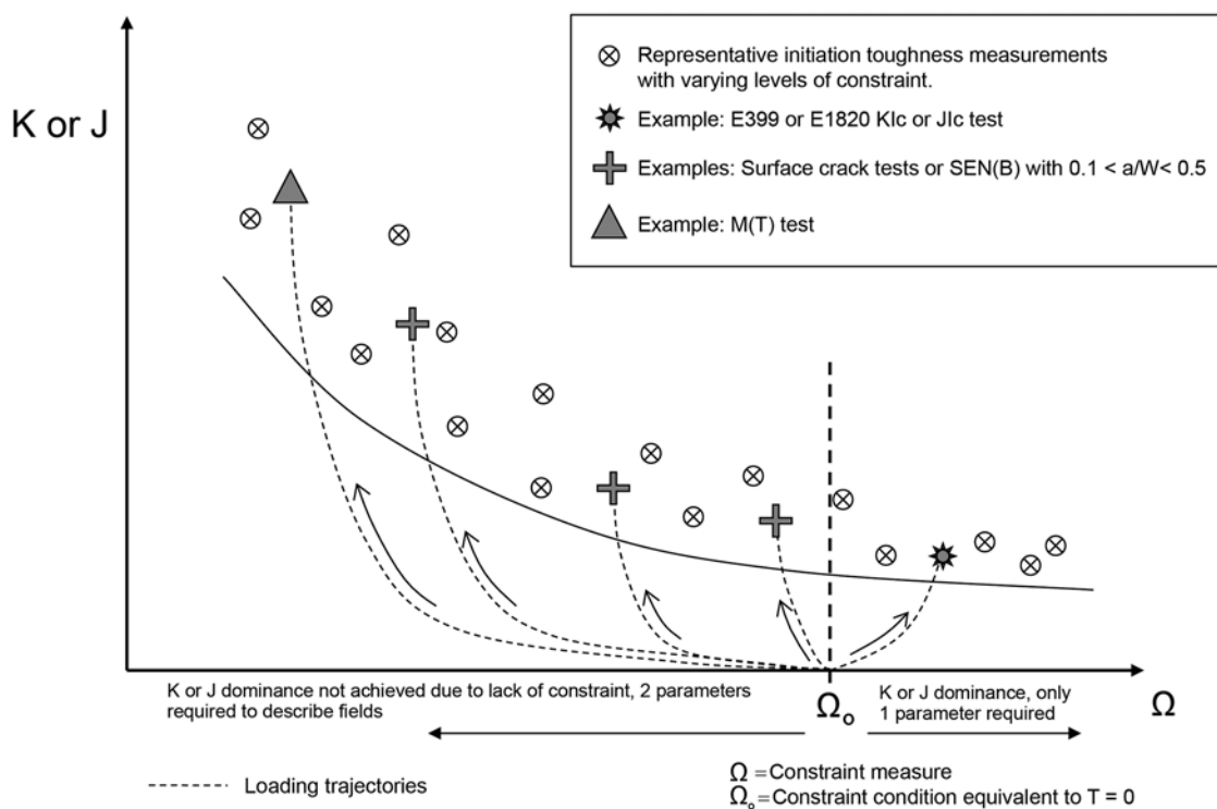
FIG. 2 Toughness-Constraint Locus with Example Trajectories
