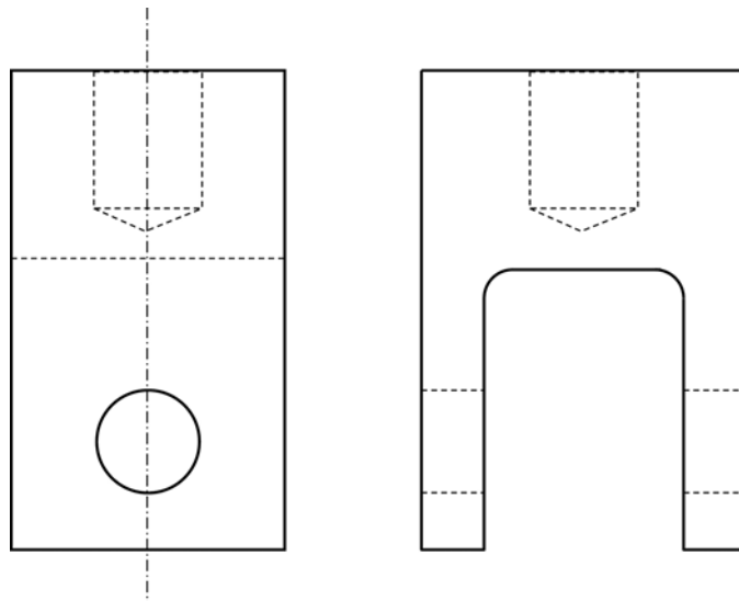
FIG. 3 Recommended configuration of tension testing clevis. Note: Flat bottomed holes are not required, but may be used in configurations found in E 1820 or E 399.
