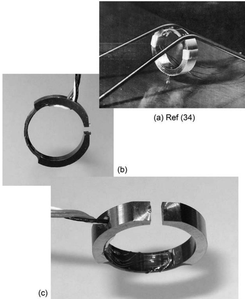
FIG. X3.2 Examples of CMOD gages and Attachments Gage designs courtesy of Ref. (33).
