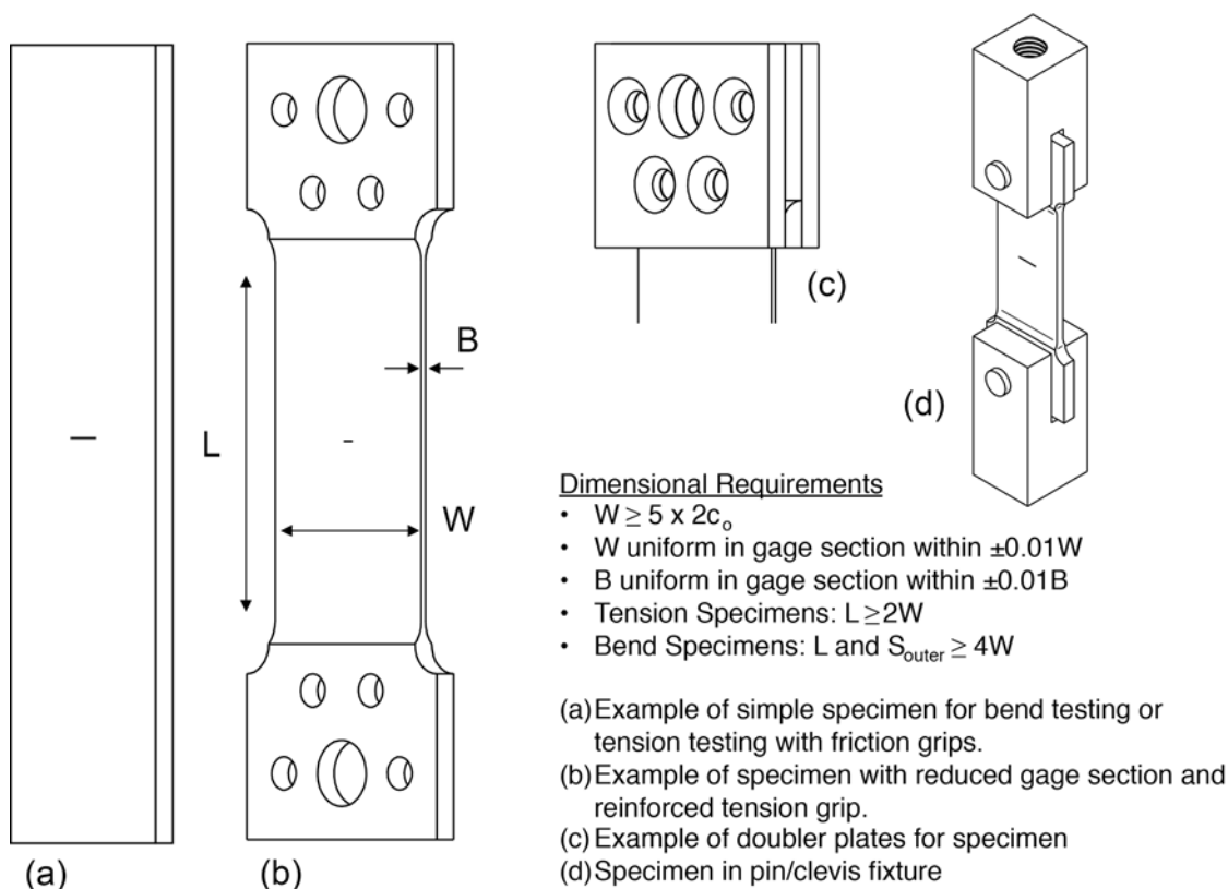
FIG. 4 Specimen Design Principles
