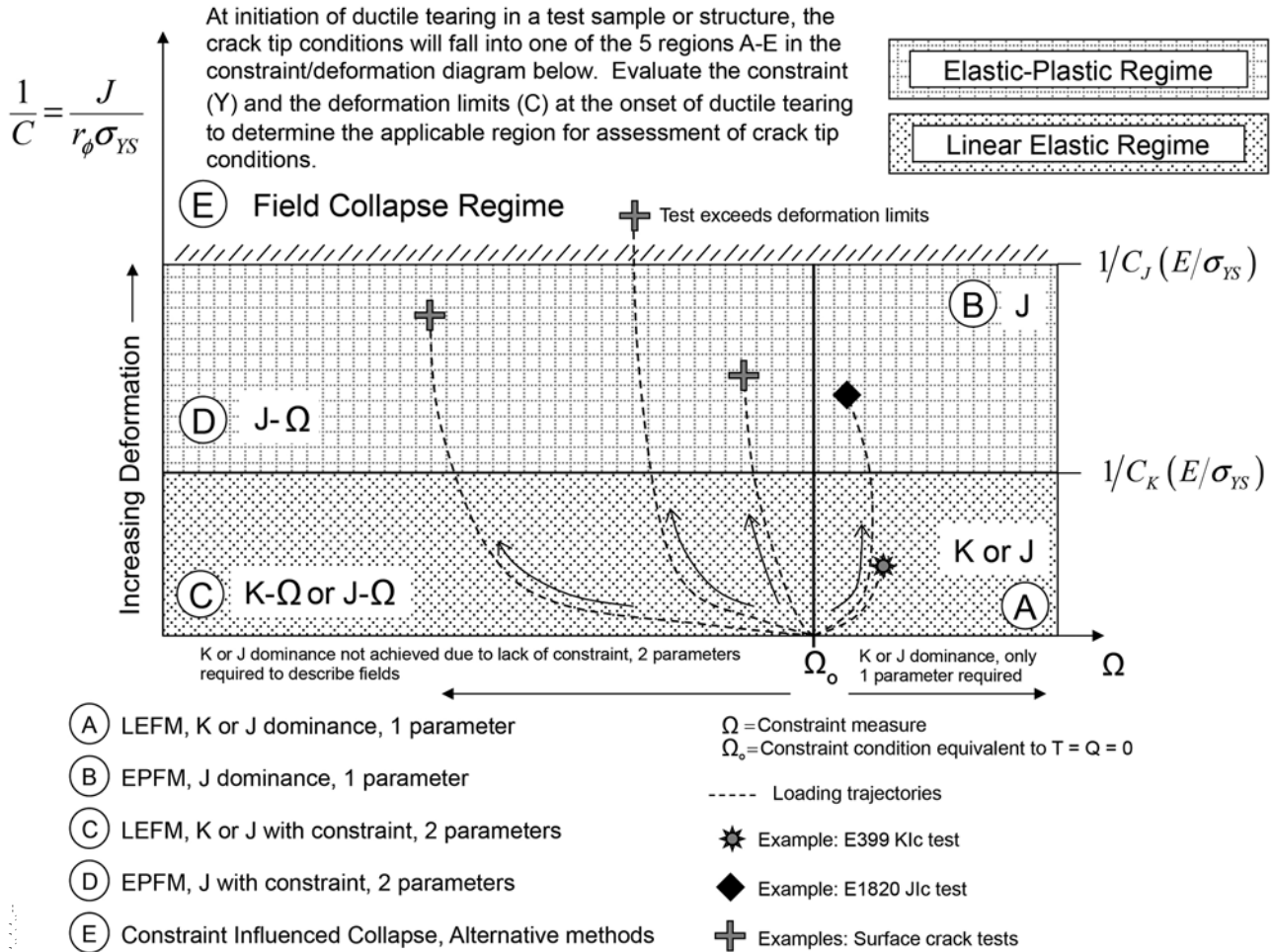
FIG. 8 Assessment of Crack Front Conditions
