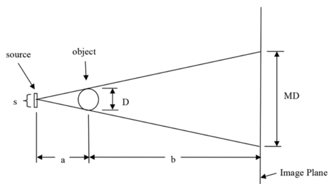
FIG. 2 Positioning of Test Object
