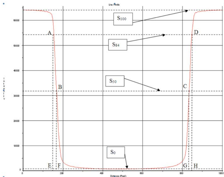
FIG. 1 Profile of Test Object Image (Test Object: Pt wire 1 mm)
