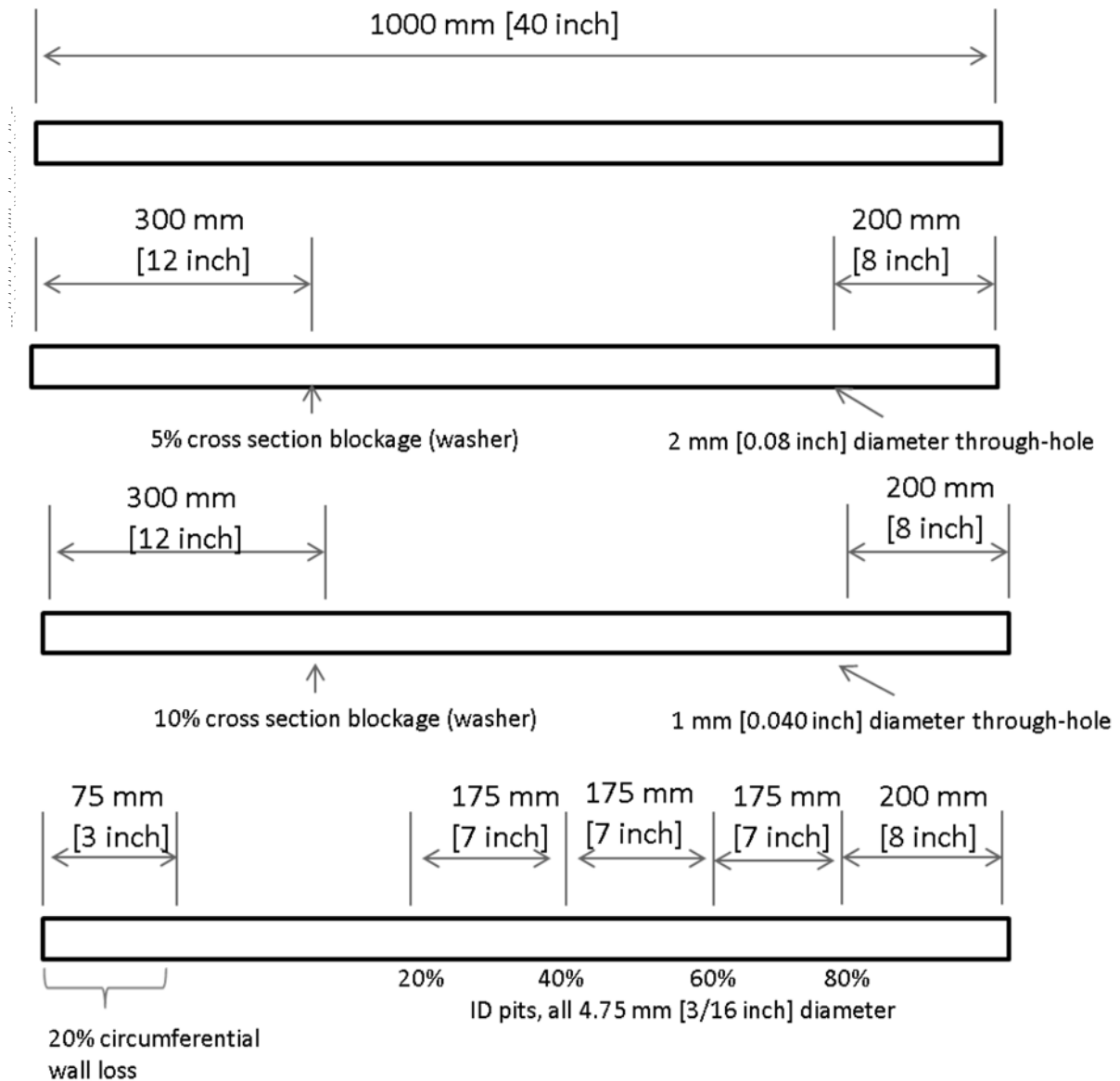
FIG. X2.1 Reference tube Specimens
