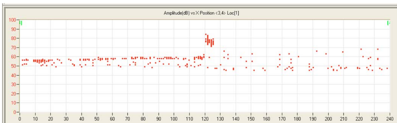
FIG. X2.1 Location Plot for 20 ft long reel spool. High amplitude source, AE indication area at “125”, was from two cracks circumferentially oriented from a balance weight mounting hole in the shell.
