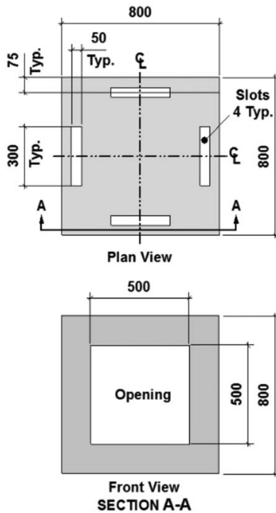
FIG. 14 Test Box for Vertical Test Assembly
