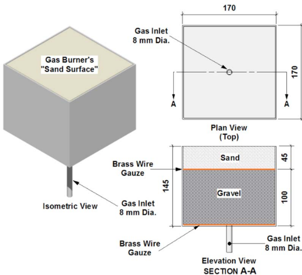
FIG. 1 Gas Burner Exposure Fire Source
