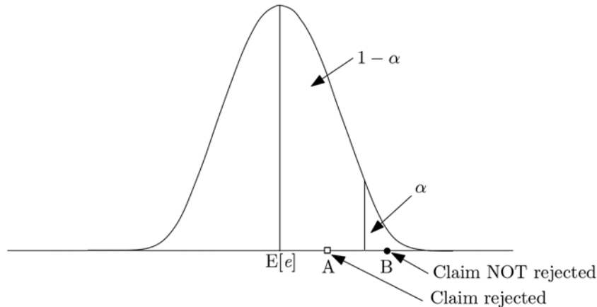
FIG. X2.1 Reject/Not Reject for the Student t -Distribution
