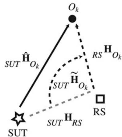
FIG. 1 Absolute Pose of Object O at Pose k Computed from the SUT Represented by {}^{SUT}\hat{\mathbf{H}}_{O_k} and Computed from the RS Represented by {}^{SUT}\tilde{\mathbf{H}}_{O_k} = {}^{SUT}\mathbf{H}_{RS} \times {}^{RS}\mathbf{H}_{O_k}
