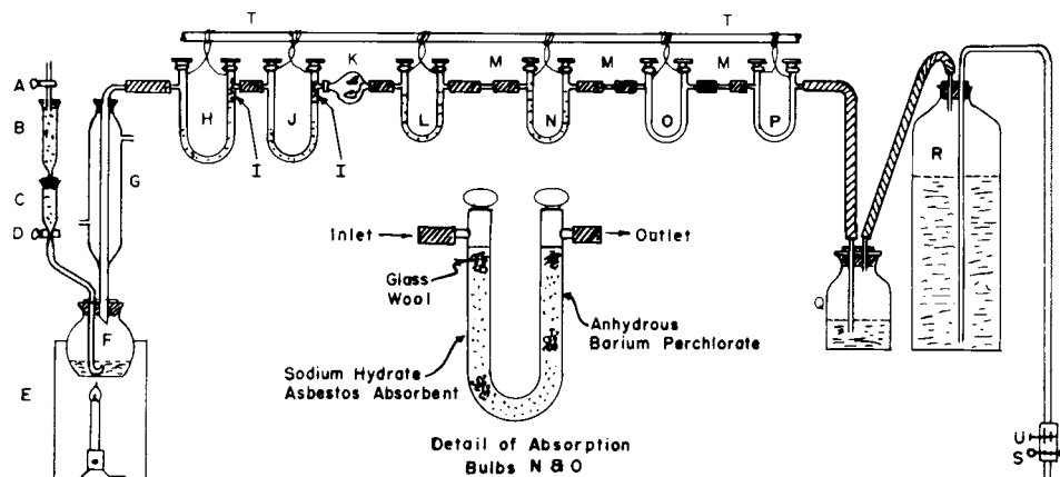
FIG. 5 Analytical Train
