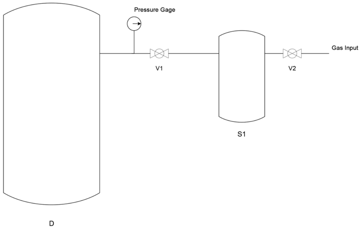
FIG. A3.2 Test System for Volume Determination
