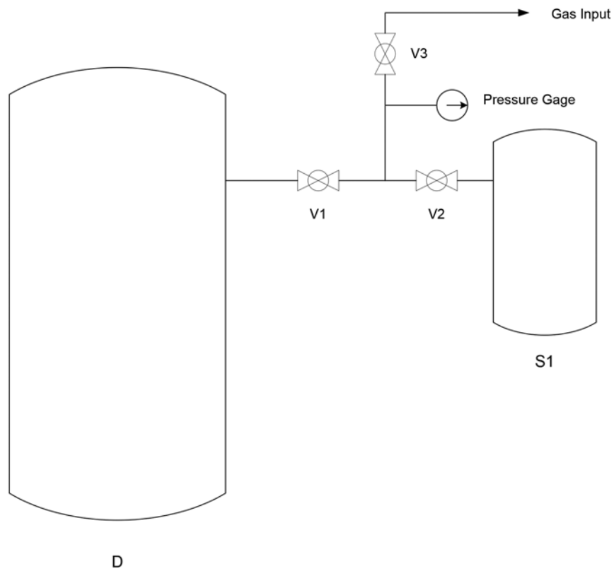
FIG. A3.3 Test System for Volume Determination with Stray Volume
