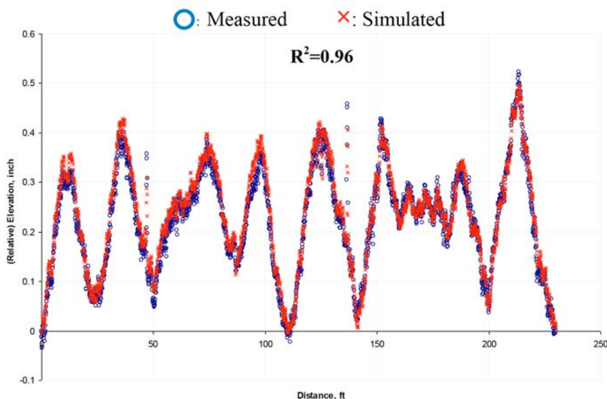
FIG. X2.1 Comparison of Profilograph Measured Profiles with ProFAA Simulated Profiles (Example)
