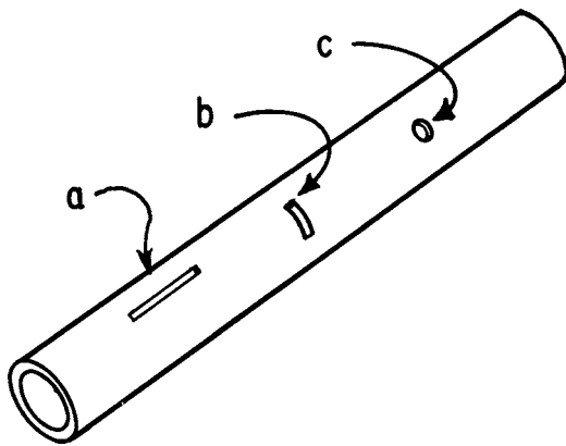
FIG. 2 Various Types of Artificial Discontinuities
