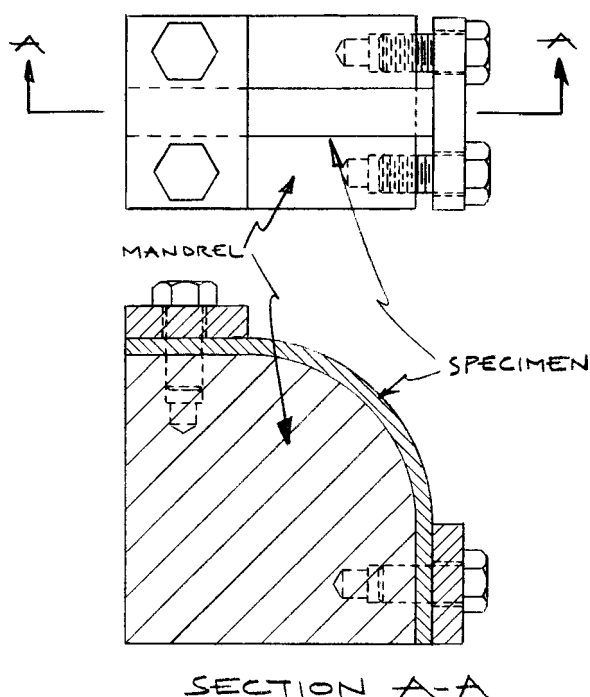
FIG. 6 Specimen in Mandrel-Type Fixture
