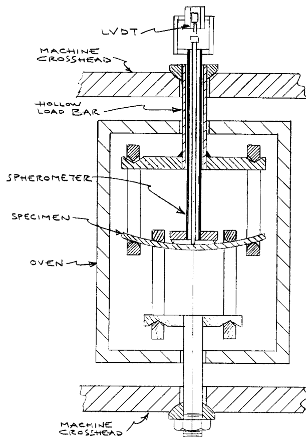
FIG. 5 Specimen and Spherometer in Four-Point Flexural Stress Fixture
