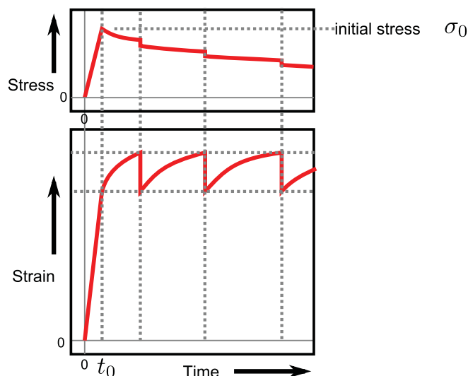
FIG. 2 Derivation of Stress-Relaxation Curve from Continuous Relaxation Technique
