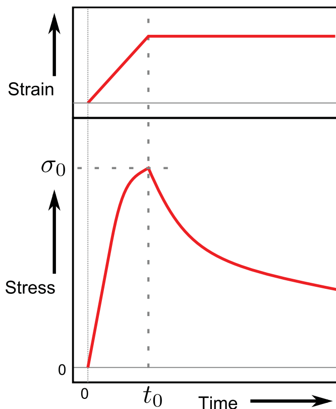
FIG. 1 Characteristic Behavior During Force Application Period in a Relaxation Test (a)
