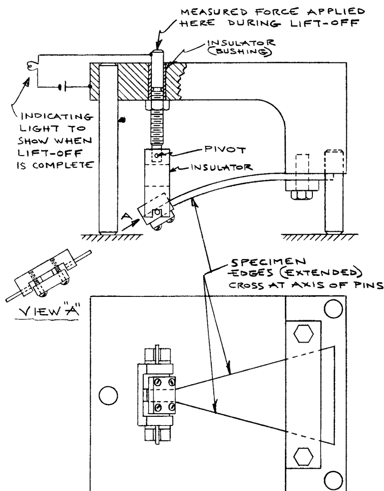
FIG. 7 Specimen in Static Fixture for Lift-Off Force Measurement
