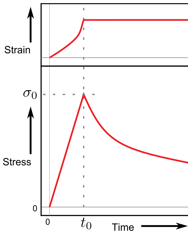
FIG. 1 Characteristic Behavior During Force Application Period in a Relaxation Test (b) (continued)
