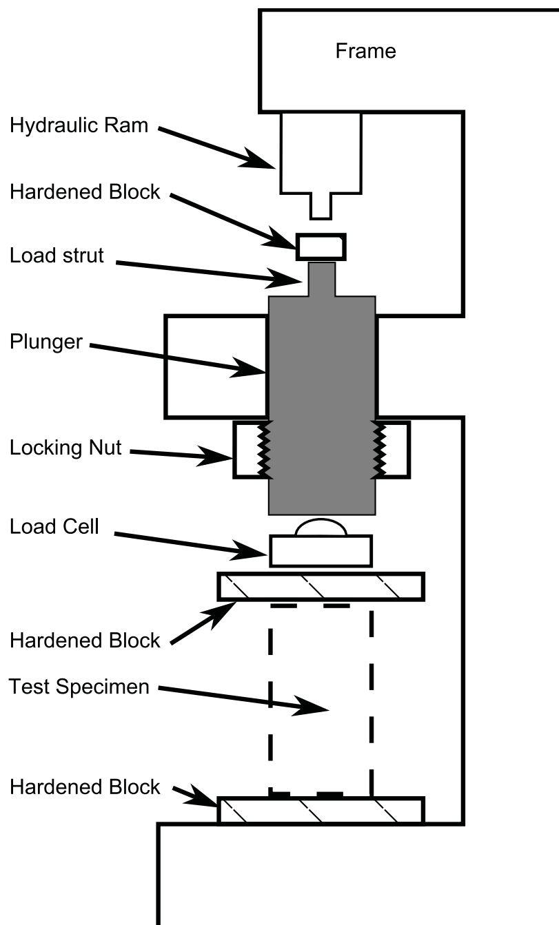
FIG. 4 Compression Stress-Relaxation Test
