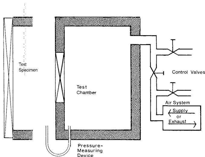
FIG. 1 General Arrangement of Testing Apparatus
