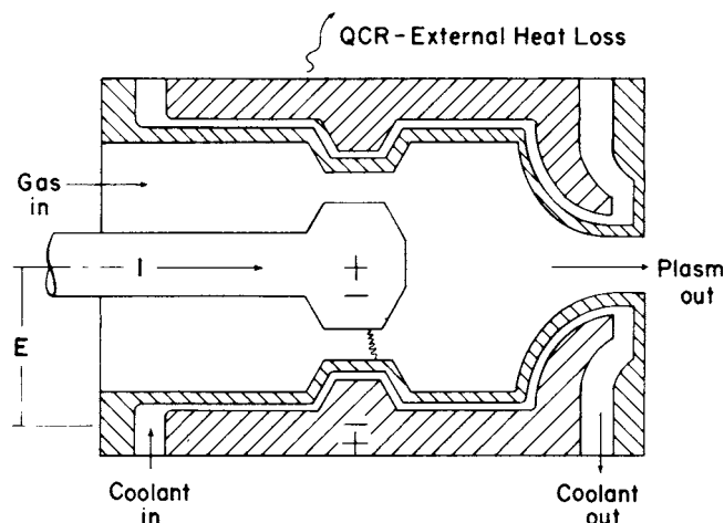
ENERGY IN – ENERGY LOSS = ENERGY TO GAS FIG. 1 Schematic Energy Balance Method for Determining Gas Enthalpy
