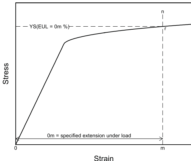
FIG. 4 Stress-Strain Diagram for Determination of Yield Strength by the Extension-Under-Load Method
