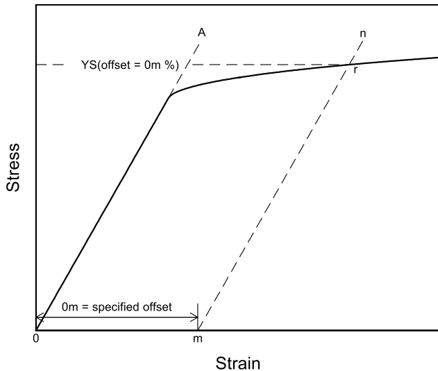
FIG. 3 Stress-Strain Diagram for Determination of Yield Strength by the Offset Method
