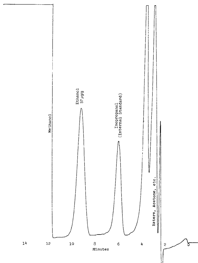
FIG. 1 Chromatogram for Refined Methanol
