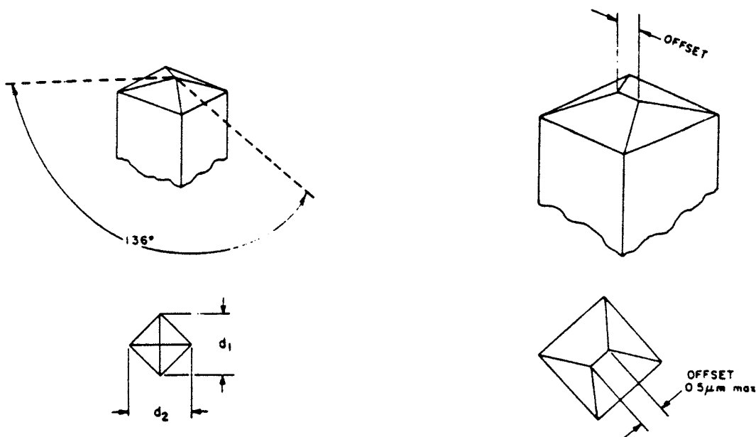
FIG. 2 Vickers Indenter
