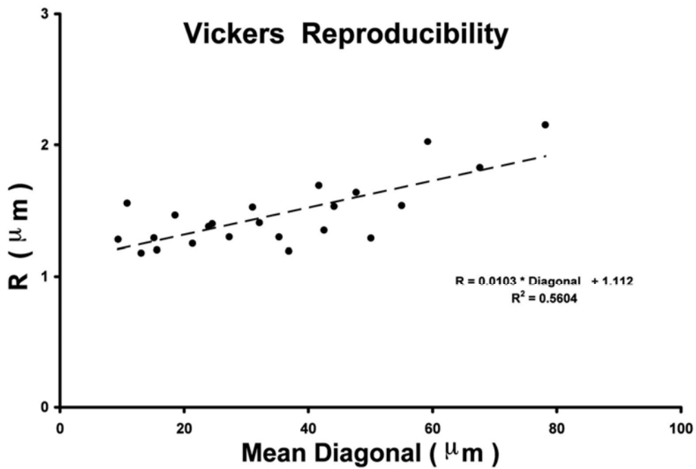
FIG. 5 The Relationship between Reproducibility and Diagonal length ( d ) from Table 5 in \mu\text{m} units, for the Vickers Hardness Tests for Specimens B, C, D, E and T
