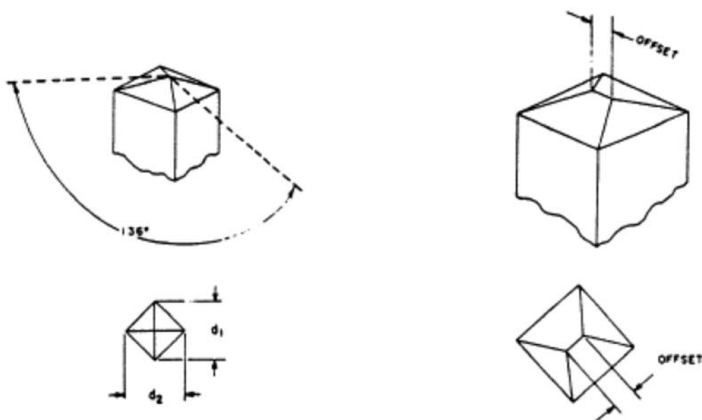
FIG. 1 Vickers Indenter
