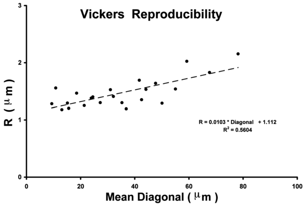
FIG. 5 The Relationship between Reproducibility and Diagonal length ( d ) from Table 8 in \mu m units, for the Vickers Hardness Tests for Specimens B, C, D, E and T
