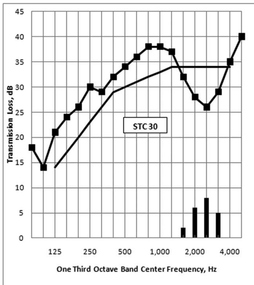
FIG. X1.2 Reference Contour (Solid Line) Fitted To Transmission Loss Data (Symbols + Line)
