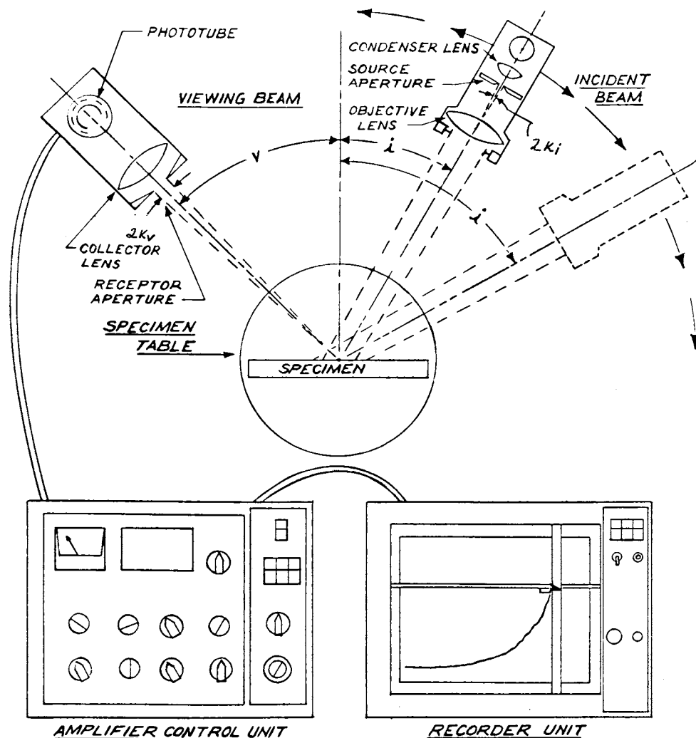
FIG. 6 Recording Goniophotometer Showing Viewing Angle, v , Incidence Angle, i , and Their Respective Field Angles, 2K_v and 2K_i
