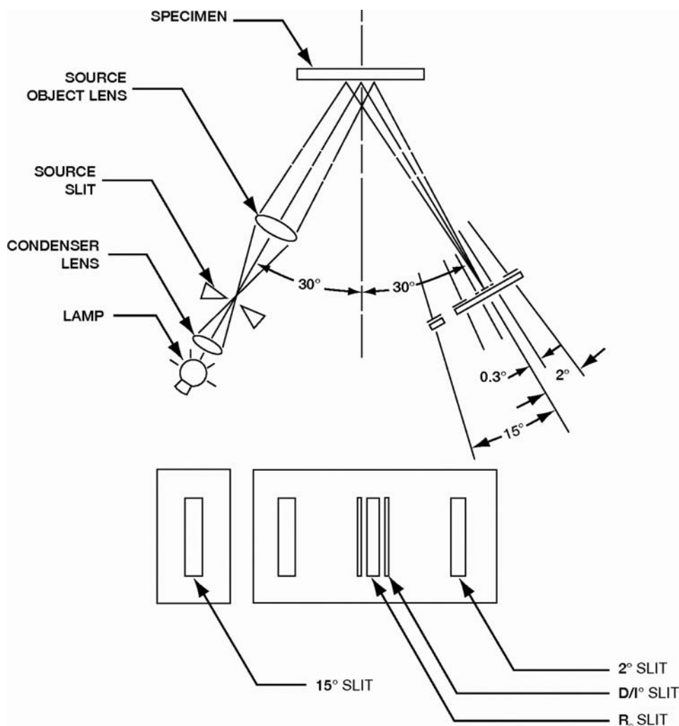
FIG. 3 Optical Diagram of the Apparatus for Method C
