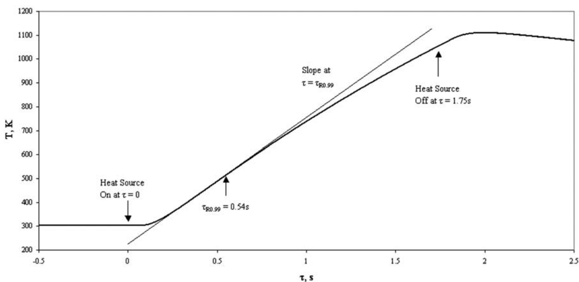
FIG. 3 Temperature–Time Curve when Heat and Other Items are Significant During Heating Phase
